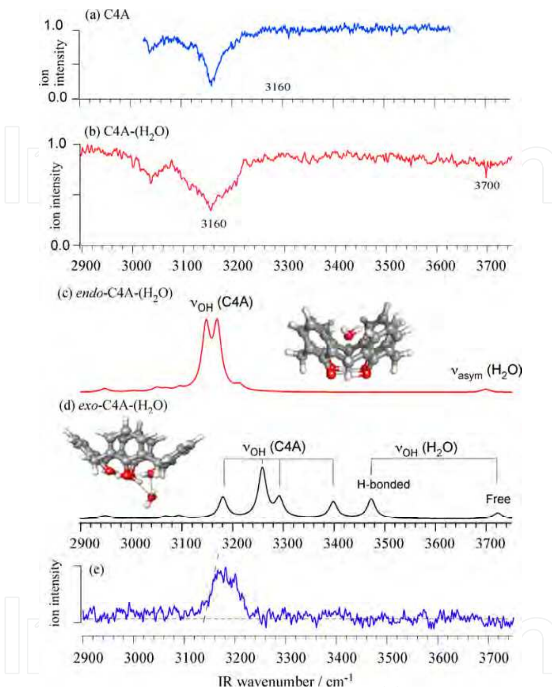
Fig. 11. IR-UV DR spectra of (a) C4A and (b) C4A-(H 2 O). Optimized structures and IR spectra of (c) endo - (Structure II) and (d) exo -form of C4A-(H 2 O) (Structure I) obtained at the MP2/aug-cc-pVDZ level of theory. (e) IRPD spectrum of C4A-(H 2 O). Figure adapted from Ref.(Hontama et al., 2010).
