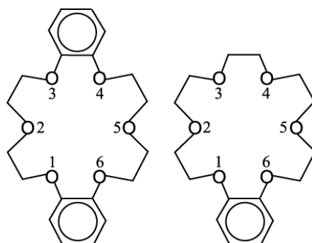
Scheme 4. Dibenzo-18-Crown-6 (DB18C6, left) and Benzo-18-Crown-6 (B18C6, right)
