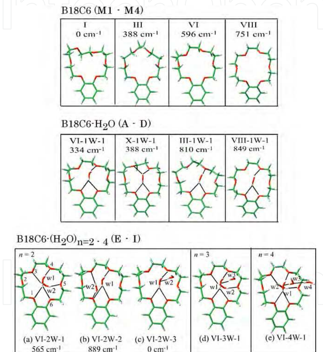
Fig. 20. (Upper) Most probable structures of B18C6 and B18C6-(H 2 O) 1 . All the calculations are done at B3LYP/6-31+G* level. (Lower) Probable structures of (a-c) B18C6-(H 2 O) 2 , (d) B18C6-(H 2 O) 3 , and (e) B18C6-(H 2 O) 4 at the B3LYP/6-31+G* level. The numbers shown in cm -1 represent the electronic energies of the isomers relative to that of VI-2W-3. Solid and dotted lines show H-bonding from the front and back sides of B18C6, respectively. Figure adapted from Ref. (Kusaka et al., 2009).
