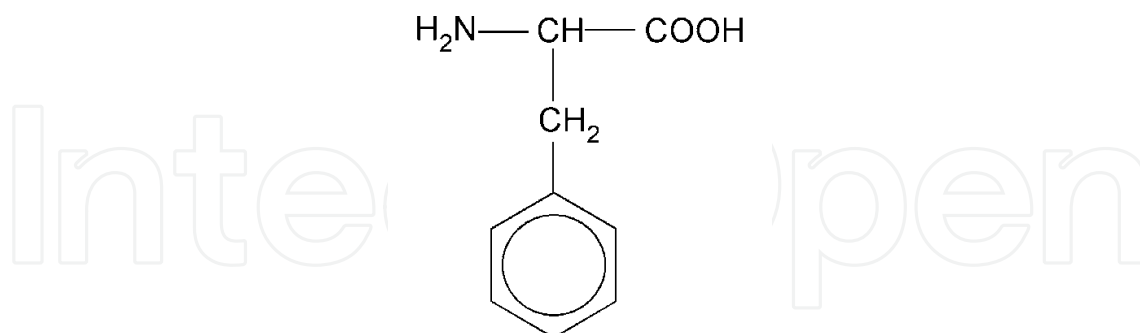
Scheme 1. L-Phenyl alanine
