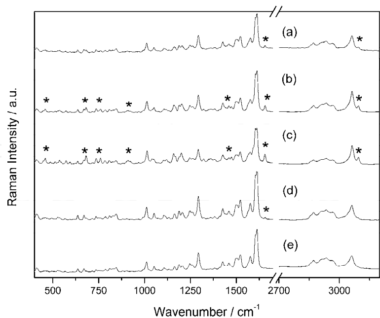
Fig. 7. Raman spectra of losartan potassium in association to chlortalidone in proportions: a) 1:1, b) 1:2, c) 1:4, d) 2:1 and e) 4:1.
