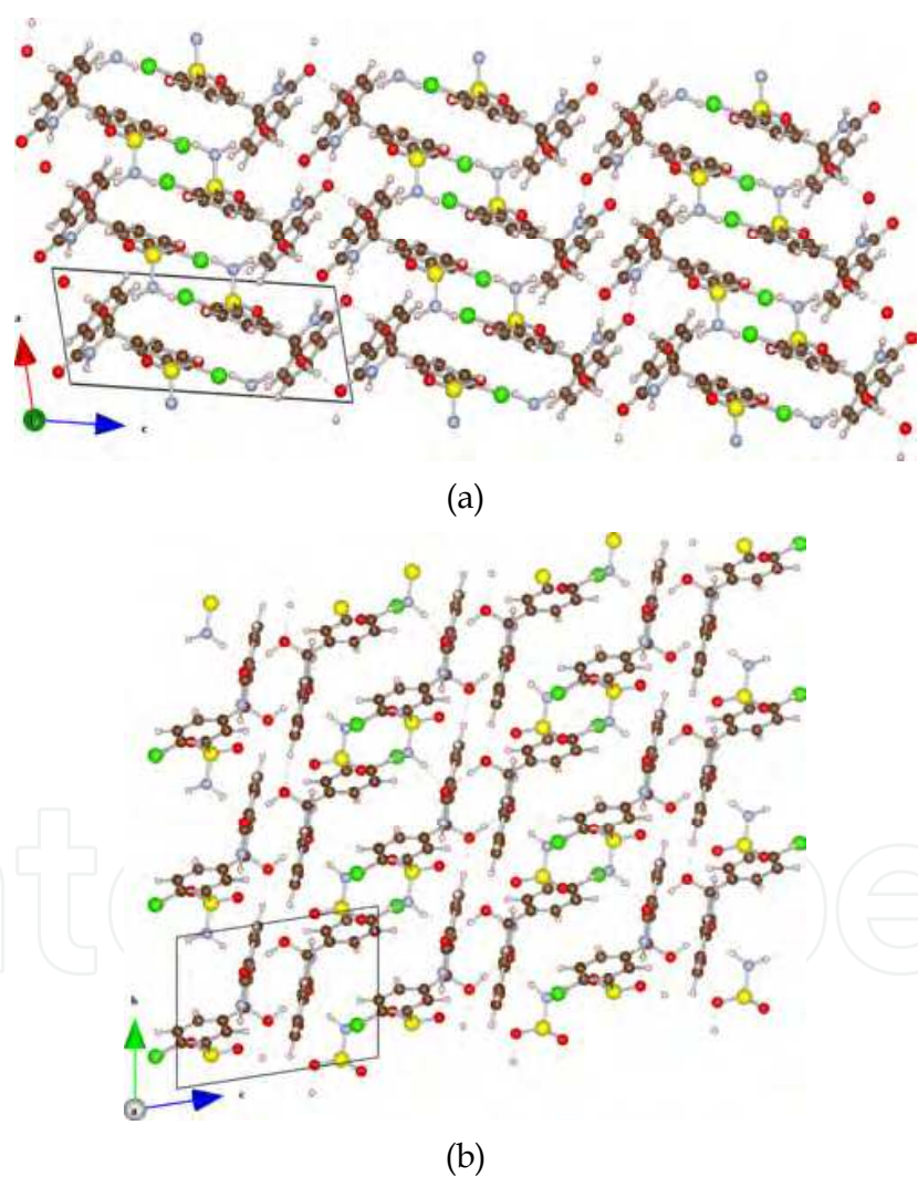
Fig. 6. Optimized structures of the chlortalidone polymorphs I (a) and III (b).
