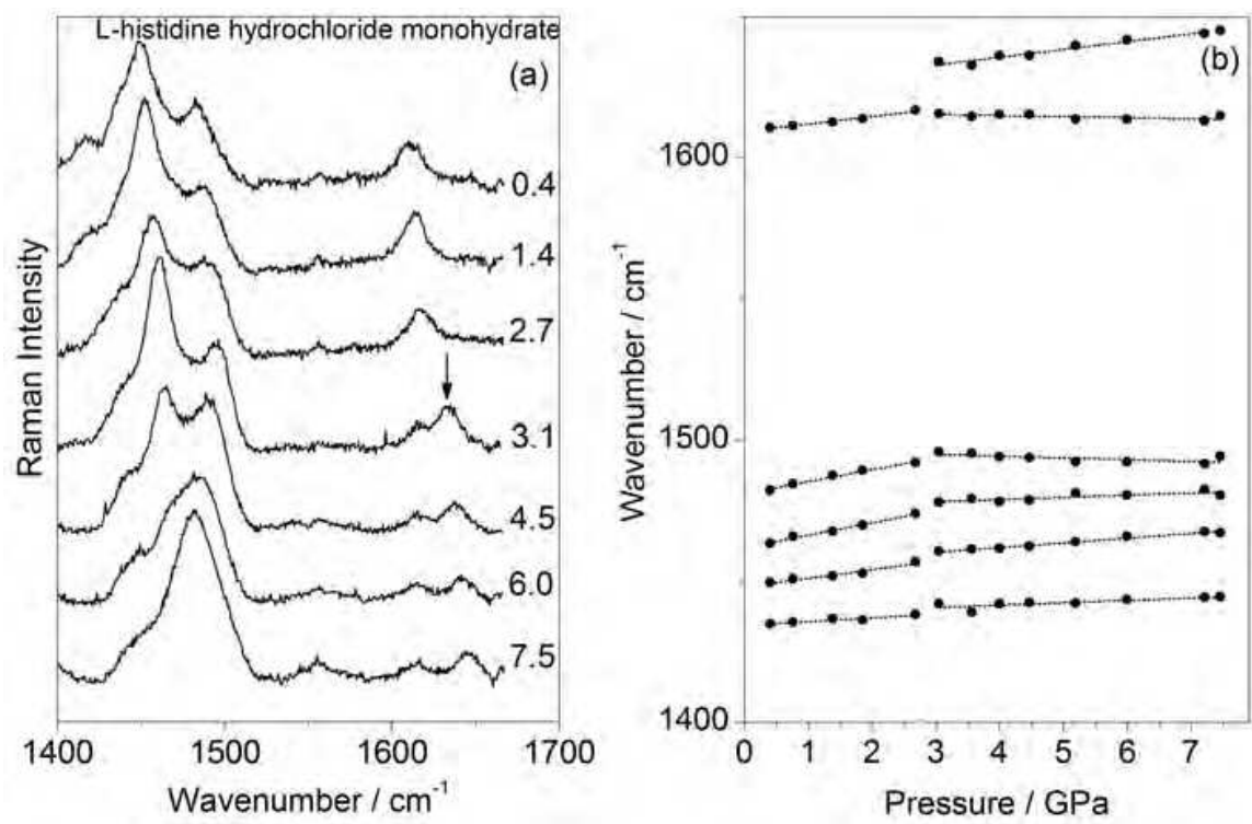
Fig. 11. (a) Raman spectra of HHM under several pressure conditions from 0.4 to 7.5 GPa in the spectral range 1400 – 1670 cm -1 ; (b) wavenumber versus pressure of the bands of HHM appearing in Fig. 11(a).
