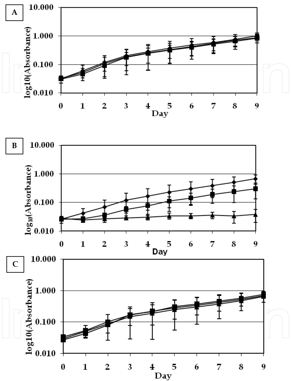
Fig. 2. Photoautotrophic Growth of Mutant and Control Strains. Growth curves showing control (diamonds) and mutant strains (R320K squares; R320D triangles) grown in either A. complete media, B. chloride-deficient media, or C. chloride-deficient media supplemented with bromide. These results are the average of at least 3 independent experiments. The error bars represent plus and minus one standard deviation.
