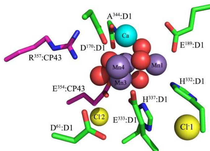
Fig. 1. Coordination Environment of the \text{Mn}_4\text{CaO}_5 Cluster.
