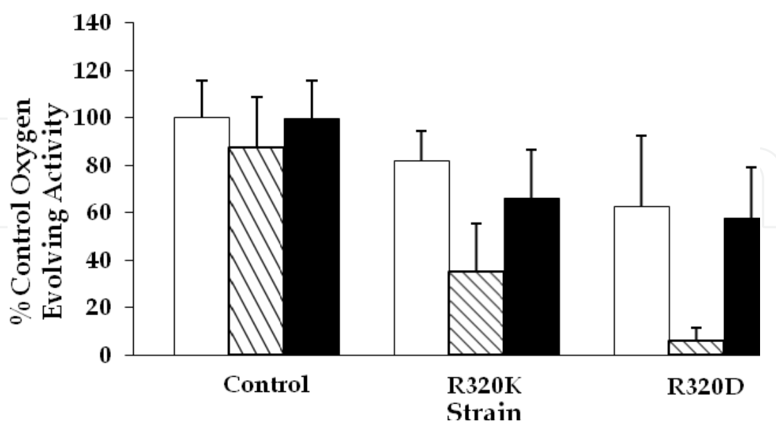
Fig. 3. Oxygen Evolution Rates of Control and Mutant Strains Grown Photoautotrophically. The control rate in complete media was 391 \mu\text{mol O}_2^*(\text{mg chlorophyll})^{-1} \text{ hr}^{-1} . Rates are expressed as the percentage of the control rate in cells grown in complete media. White bars, oxygen evolution rates from cells grown in complete media; Striped bars, oxygen evolution rates from cells grown in chloride deficient media; Black bars, oxygen evolution rates from cells grown in chloride depleted media with 480 \mu\text{M} bromide added. The results are the average of at least three independent experiments. The error bars represent plus and minus one standard deviation.
