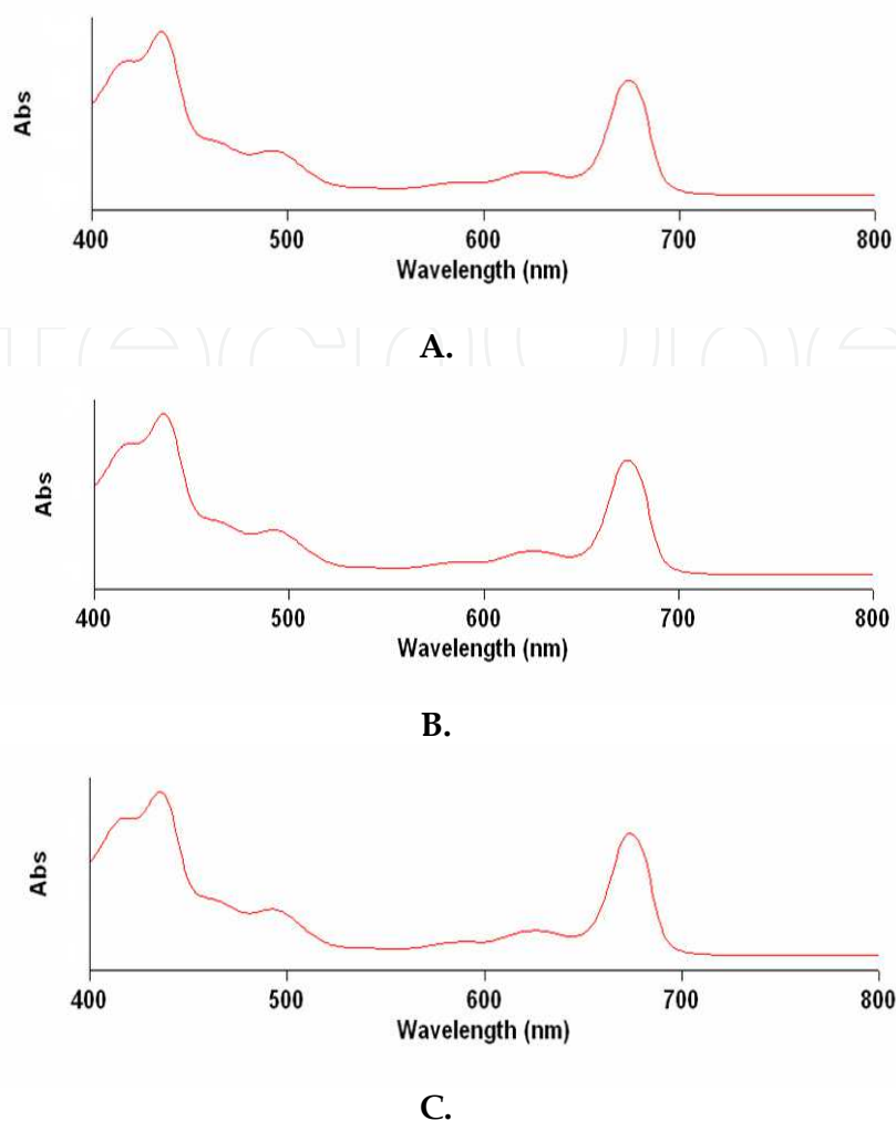
Fig. 4. Visible Absorption Spectra
