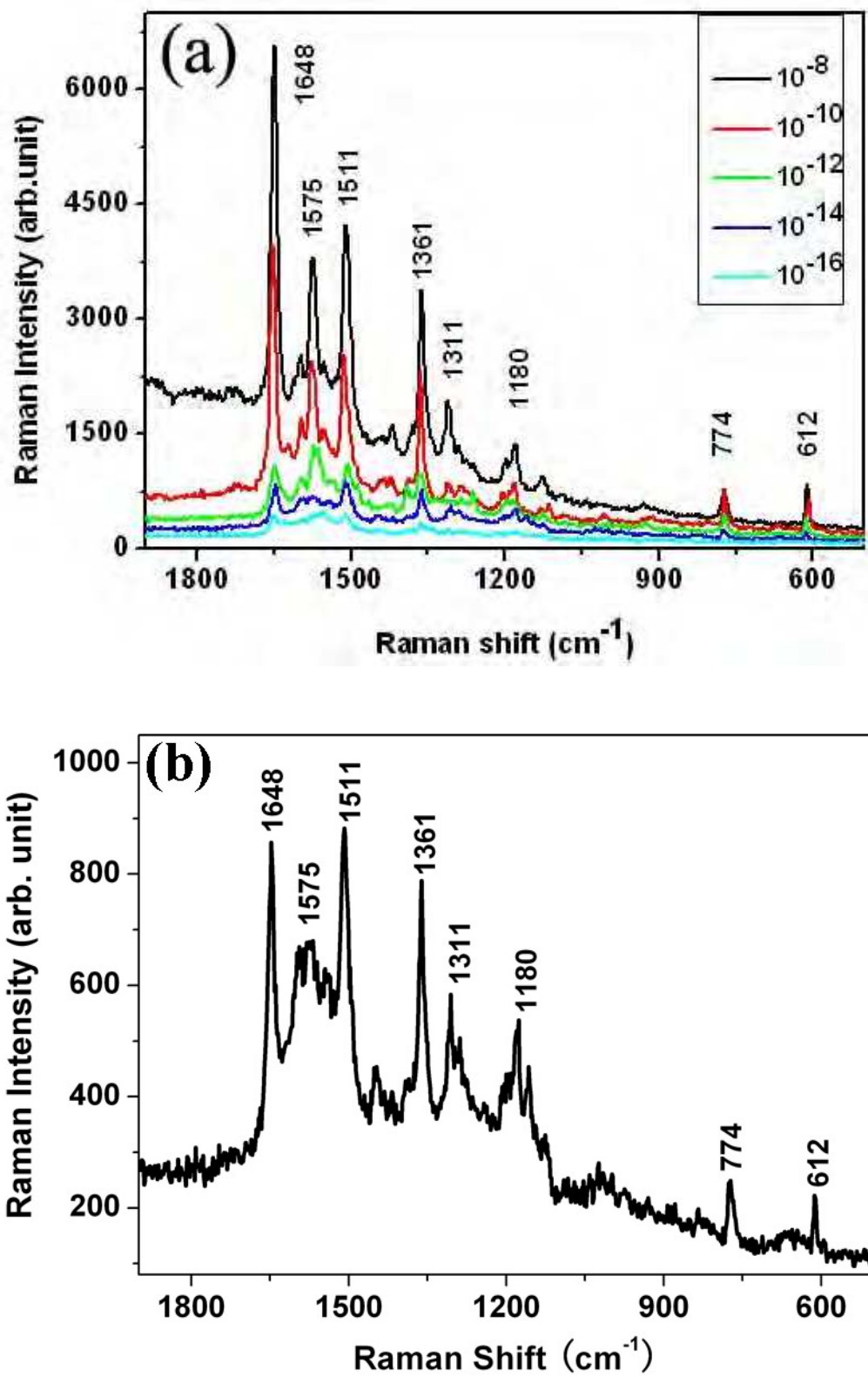
Fig. 4. (a) Raman spectra of R6G at concentrations ranging from 1x10 -8 to 1x10 -16 mol/L; and (b) the Raman spectrum of R6G at a concentration of 1x10 -14 mol/L, on the thin Ag film consisting of well separated, single crystalline Ag nanorods.
