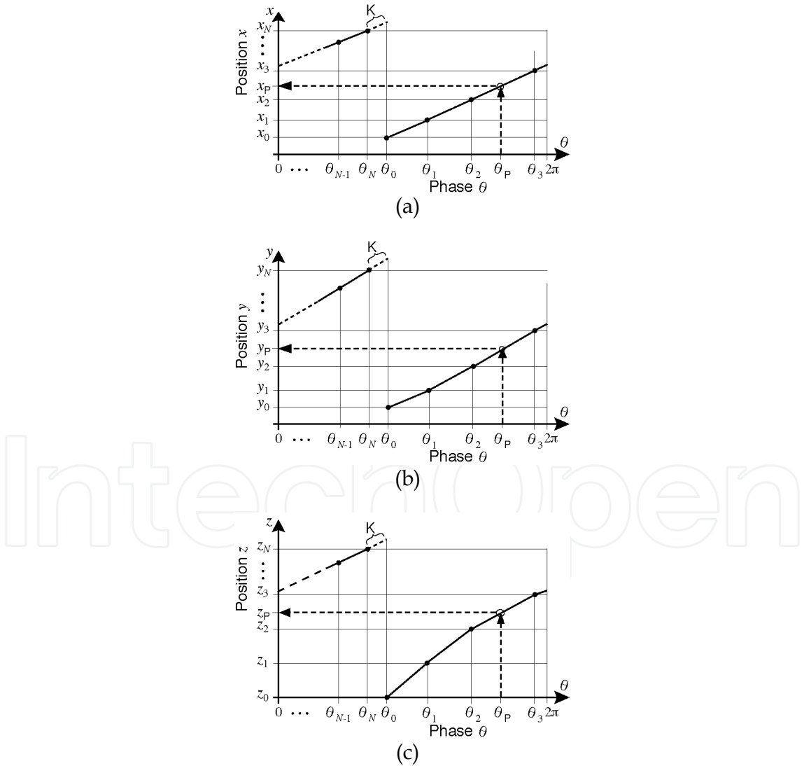
Fig. 4. Calibration tables to obtain x , y and z coordinates from phase at each pixel point of camera; (a) Table of phase \theta and x ; (b) Table of phase \theta and y ; (c) Table of phase \theta and z
