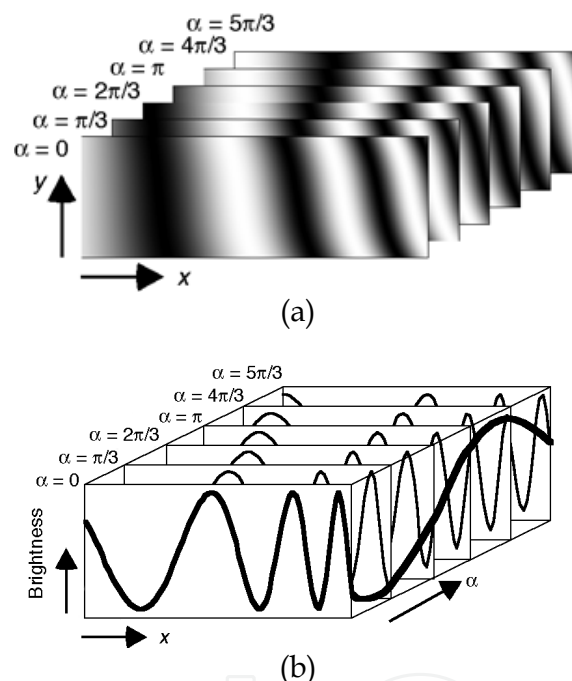
Fig. 2. Phase analysis of projected grating using phase-shifting grating images; (a) Phase-shifted grating pattern projected onto object; (b) Brightness distribution along horizontal center line of Fig. (a)
