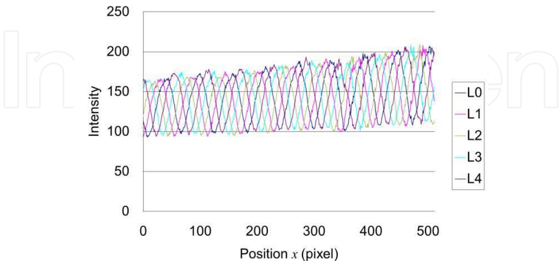
Fig. 9. Intensity distributions along x-axis of projected grating on reference plane when changing light sources
