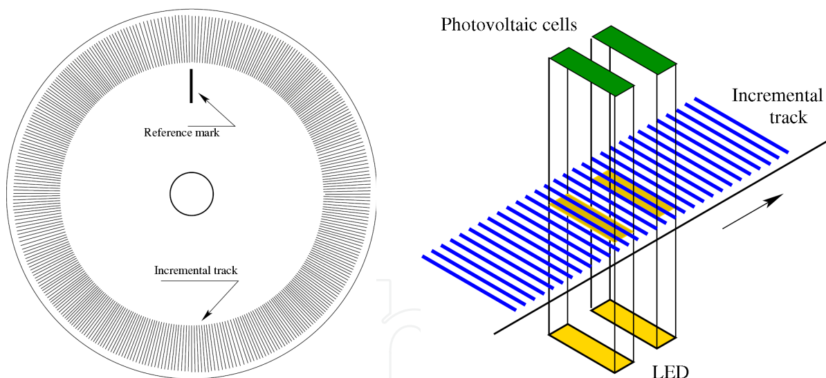
Fig. 7. The optical angle encoder.
