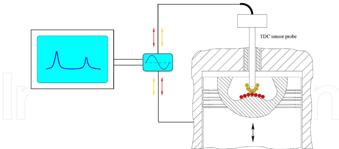
Fig. 8. The capacitive TDC sensor.
