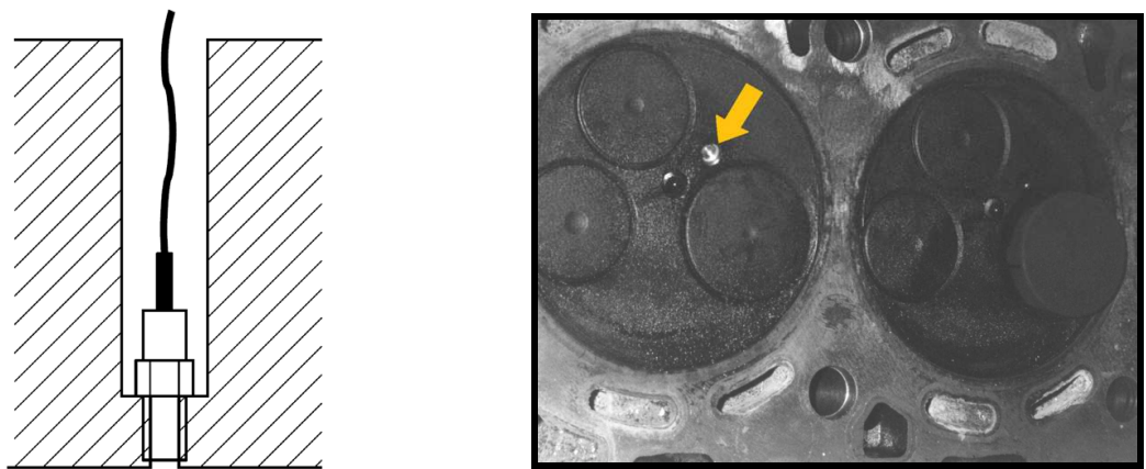
Fig. 3. Pressure transducer mounting location.
