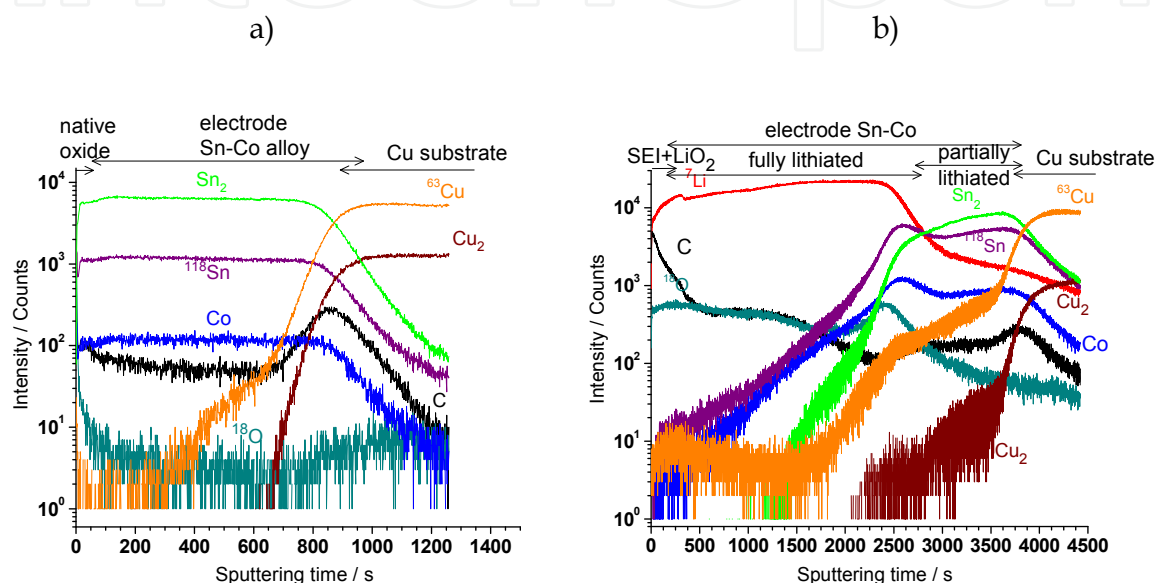
Fig. 3. ToF-SIMS negative ion depth profiles of (a) pristine and (b) lithiated Sn-Co alloy electrode at 0.02 V vs Li/Li + in 1M LiClO 4 /PC.
