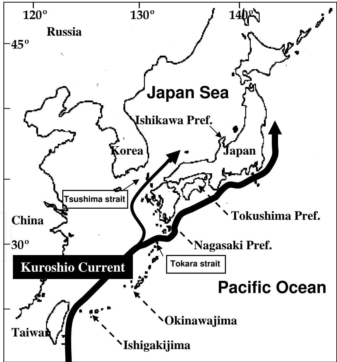
Fig. 7. The location of the main pathway of Kuroshio Current and sampling sites.
