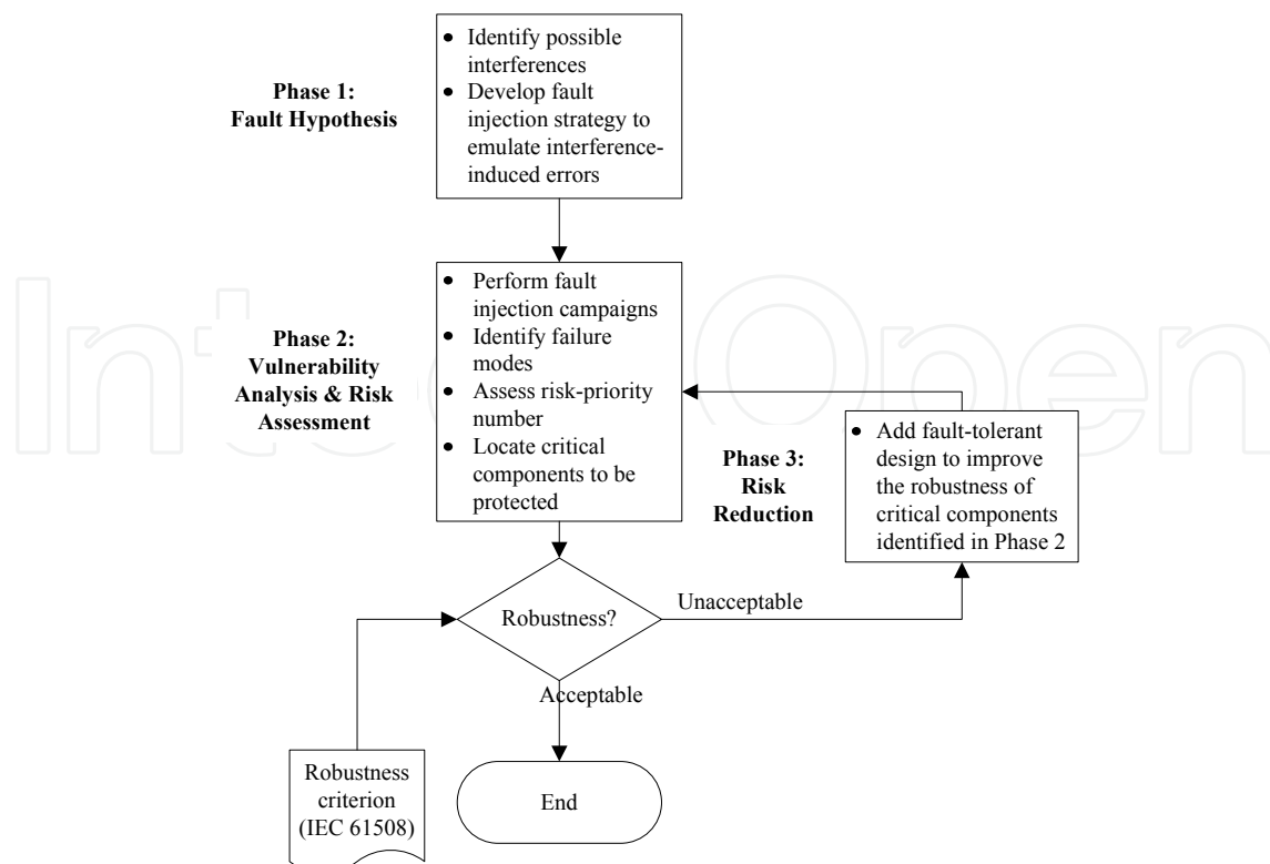
Fig. 1. Safety validation and risk reduction process.
