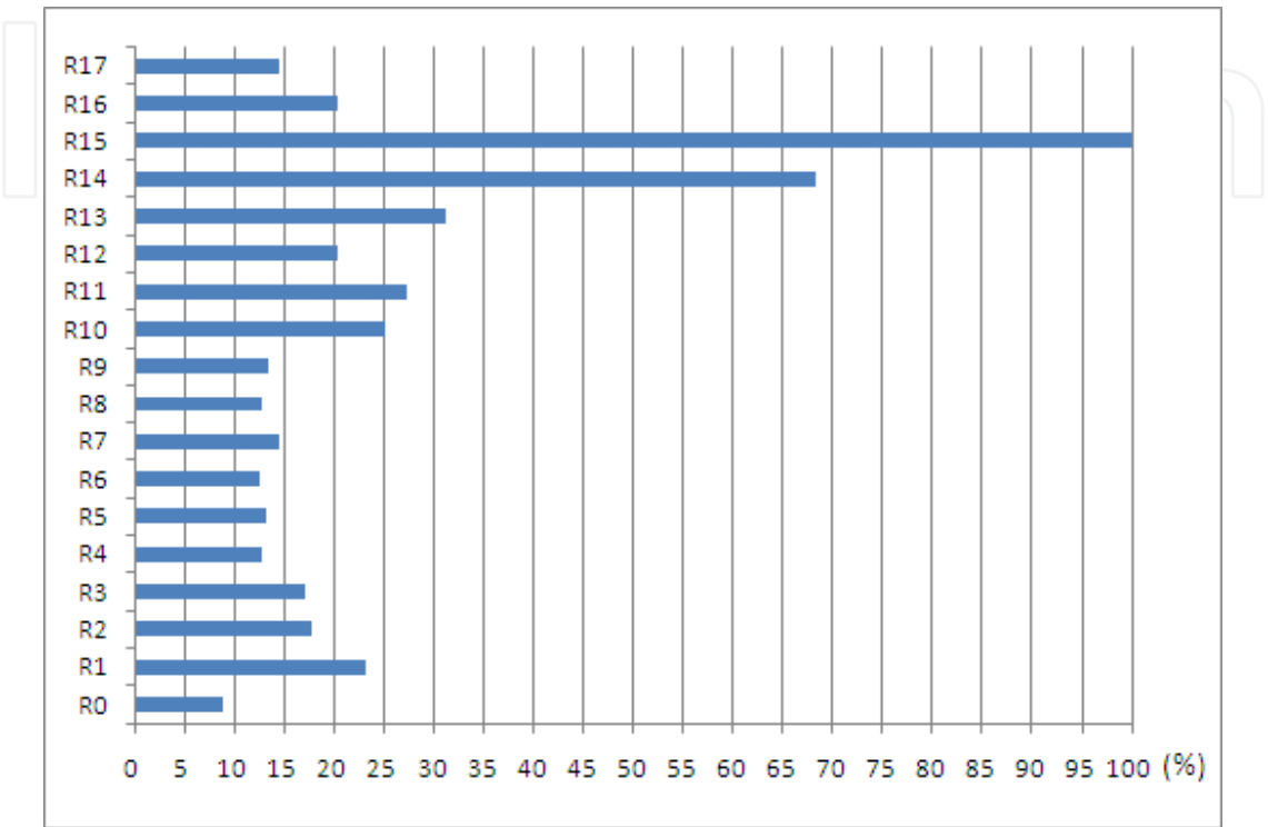
Fig. 2. The average SoC failure probability from the data of the used benchmarks.
