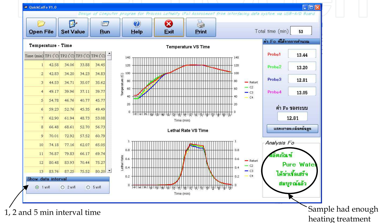
Fig. 18. The result displayed by QuickCalFo
