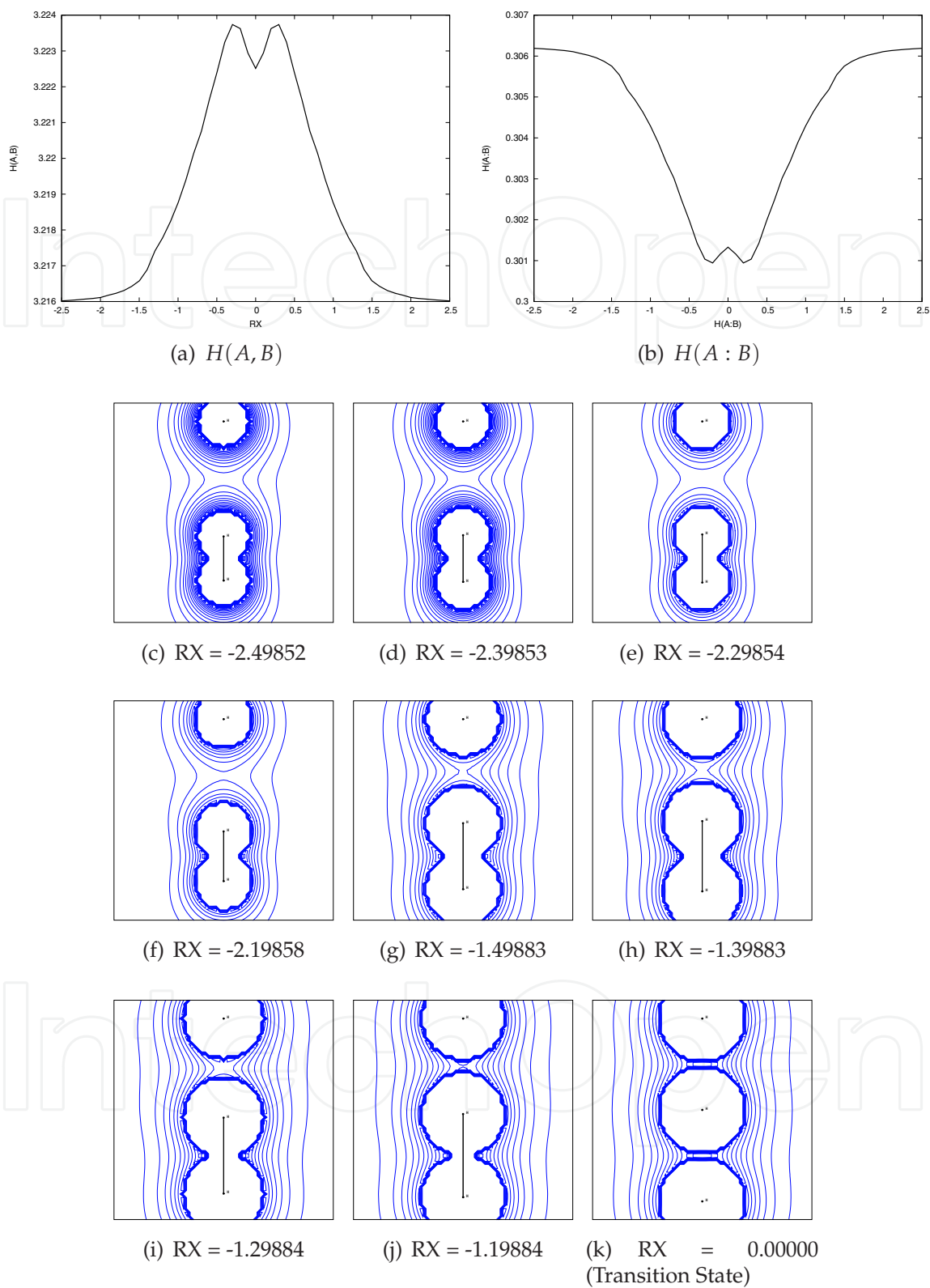
Fig. 6. Trends of H(A,B) , H(A : B) using \{A\} = \{H\} and \{B\} = H_{in}H_{out} and the Molecular Electric Potential in different points of the reaction coordinate in the process H_2 + H^- \longrightarrow H_2 + H^- .
