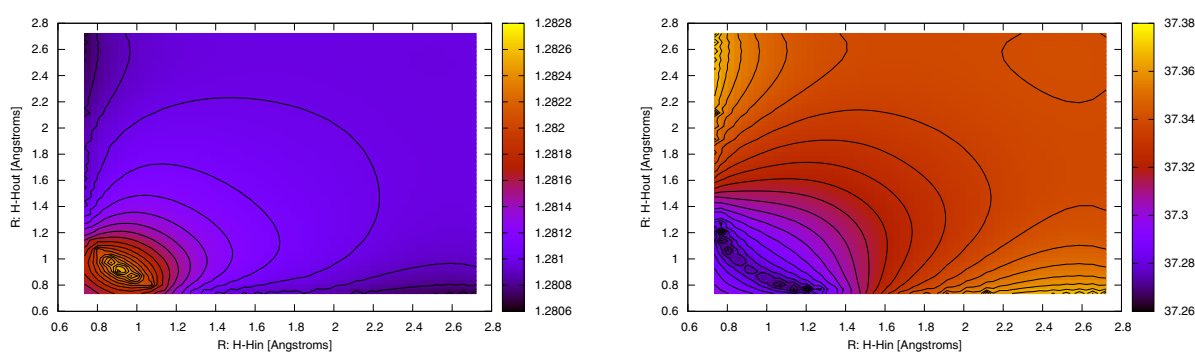
(a) Internuclear distances with informational flow (b) Inter nuclear distances with informational trajectory
