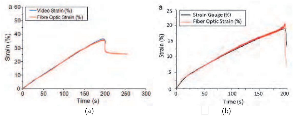
Fig. 16. Plot showing the response of the POF sensor during a quasi-static tensile loading for (a) a non-woven specimen, (b) a woven specimen (after [16]).
