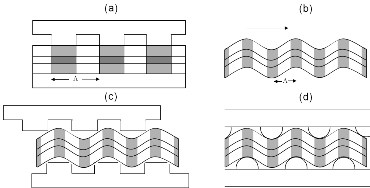
Fig. 3. Stress induced LPFGs, pressure points (a,b) microbending (c,d)
