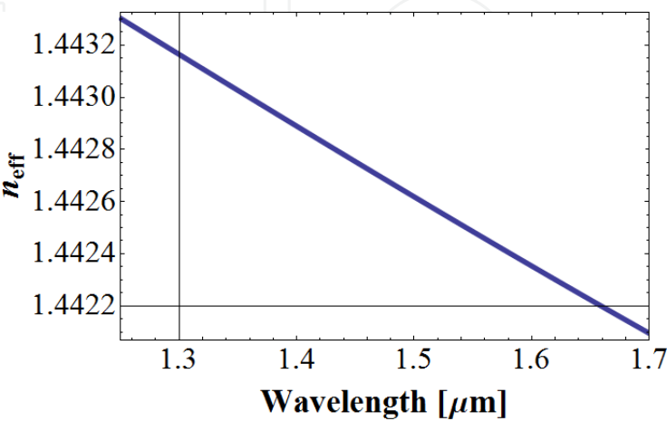
Fig. 5. Effective index of the fundamental core mode as a function of wavelength.
