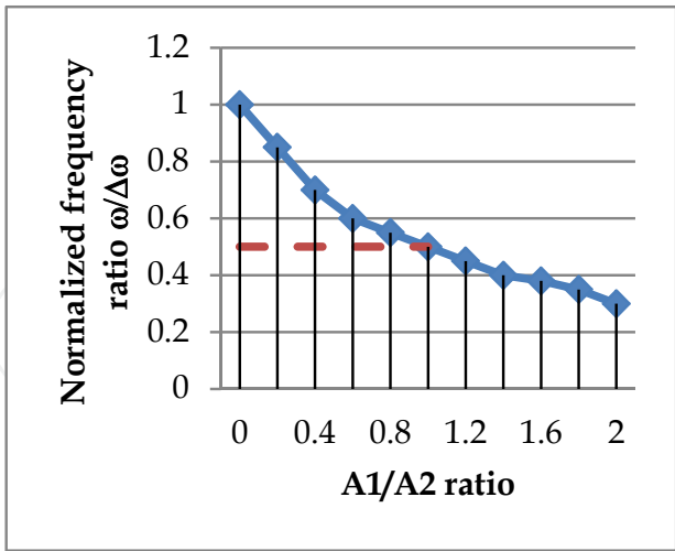
Fig. 8. Dependence |\omega/\Delta\omega|(A_1/A_2)
