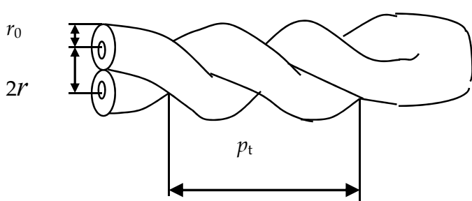
Fig. 14. Structure of sensor part
