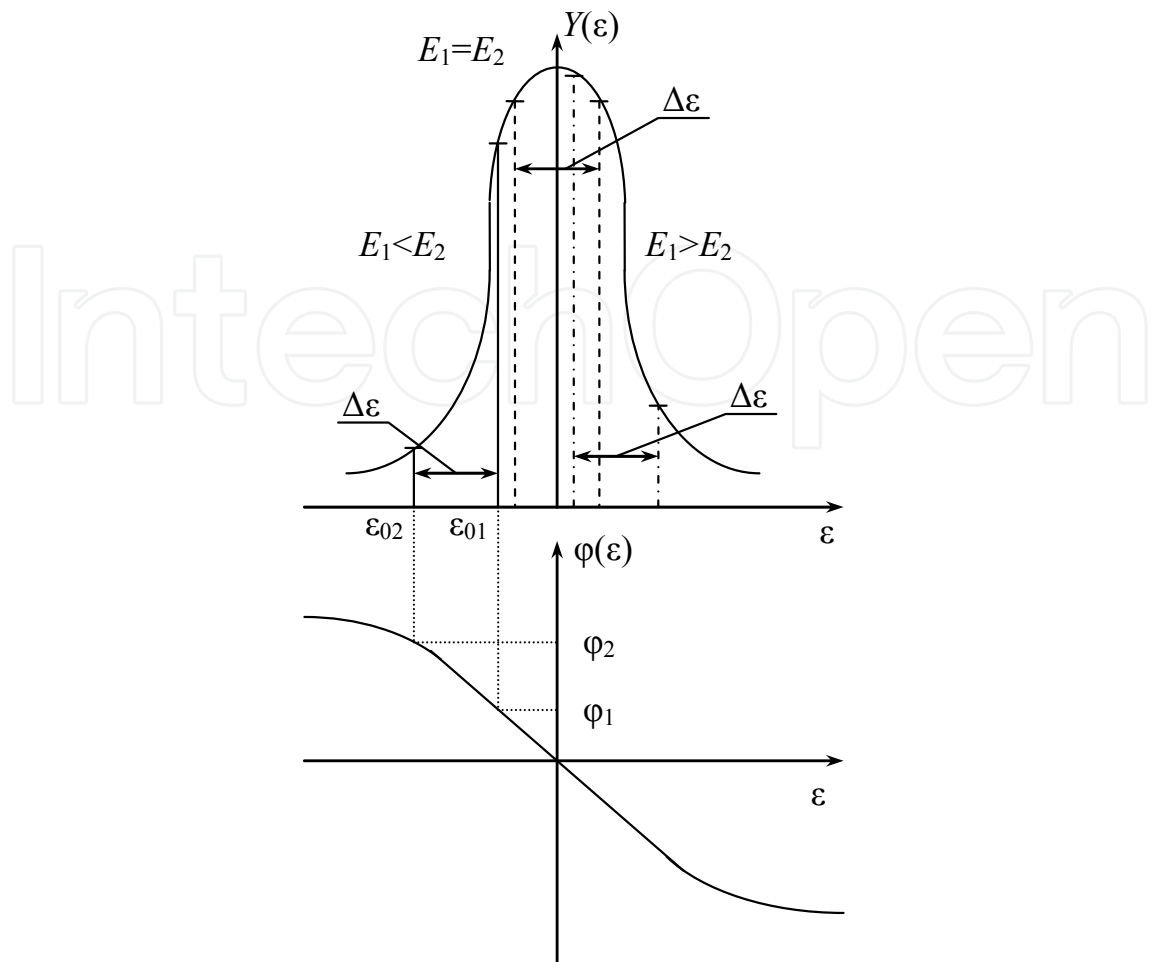
Fig. 16. Circuit amplitude-frequency characteristic with two-frequency input signal
