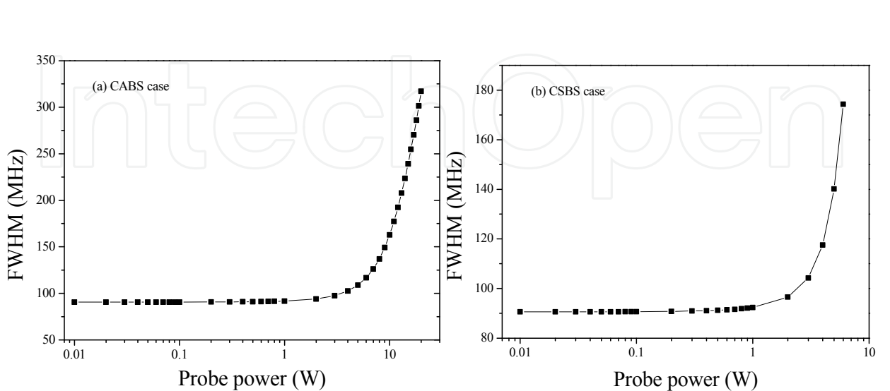
Fig. 9. Spectrum width as a function of probe power for (a) coherent anti-Stokes Brillouin scattering (CABS) and (b) coherent Stokes Brillouin scattering (CSBS).
