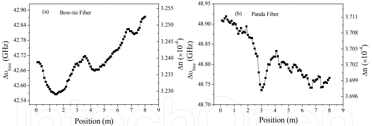
Fig. 16. Measured distributed birefringence of (a) a 8-m Bow-tie fiber and (b) a 8-m Panda fiber. (Dong et al., 2010a, with permission from OSA)
