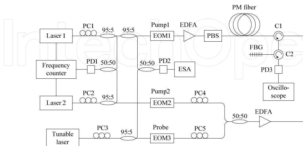
Fig. 11. Experimental setup. PC: polarization controller, EOM: electro-optic modulator, PBS: polarization beam splitter, C: circulator, PD: photo-detector, EDFA: Erbium-doped fiber amplifier, ESA: electrical spectrum analyzer, FBG: fiber Bragg grating.
