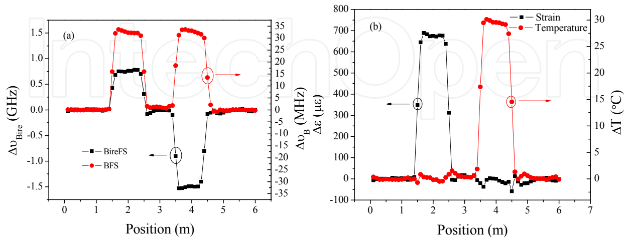
Fig. 19. (a) Measured birefringence-induced frequency shift (BireFS) and Brillouin frequency shift (BFS) and (b) calculated temperature and strain. (Dong et al., 2010c, with permission from IEEE)
