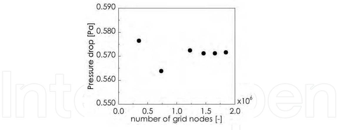
Fig. 15. Dependency between pressure drop and number of grid nodes in the CFD analysis for case-I
