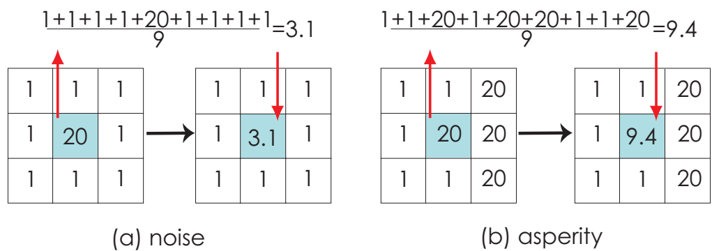
Fig. 9. Procedure of Moving-Average Algorithm for 3 × 3 Cubes
