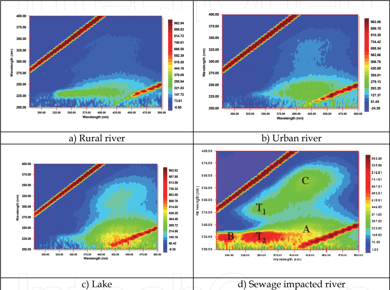
Fig. 6. Fluorescence excitation –emission matrix for water samples.
