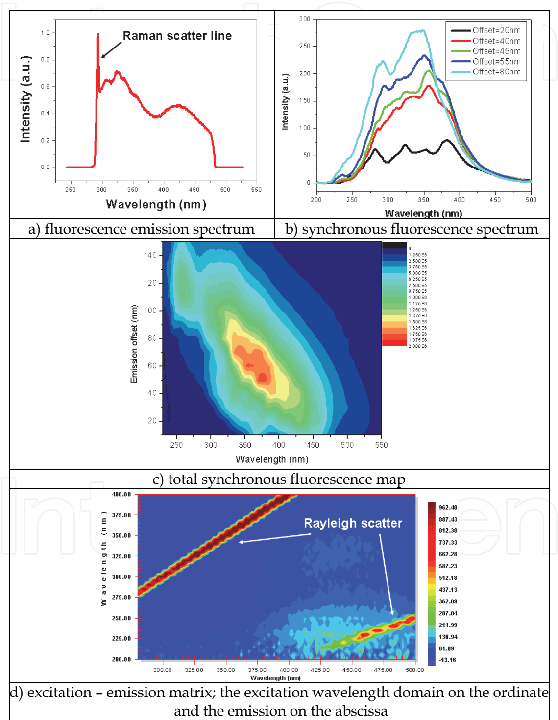
Fig. 3. Typically recorded fluorescence spectra for water samples
