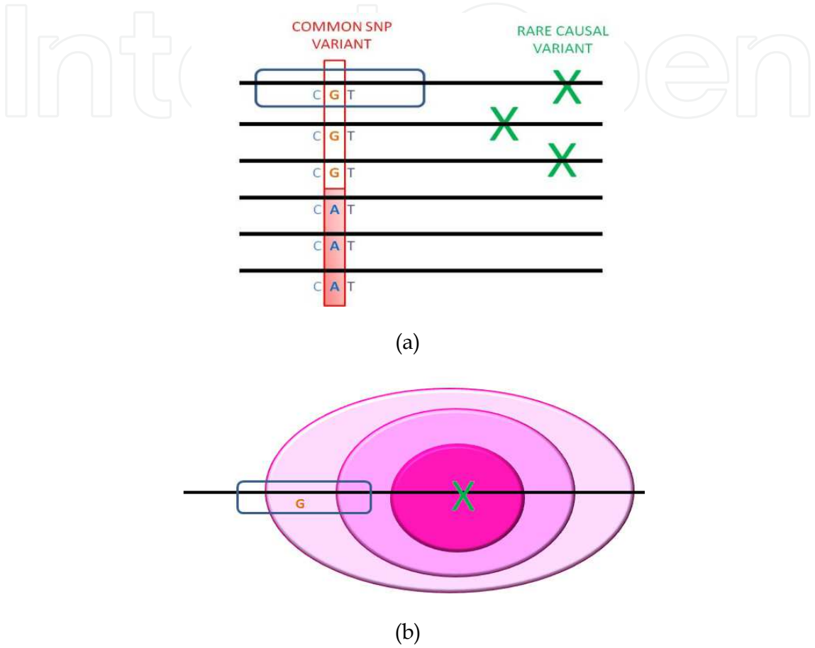
Fig. 2. (a) Synthetic Associations occur when causal rare variants are inherited more commonly with one tag SNP allele (e.g. “G”) than the other (“A”) allele (black lines represent different individuals). This rare variant may be outside the region of linkage disequilibrium defined by the common SNP (shown by the blue box). Adapted from (Cirulli et al. 2010). (b) Because the rare variant is too infrequent to be detected by GWAS, the true strength of the association signal will be missed. A diluted version of this signal will instead be represented by the common variant (Dickson et al. 2010).
