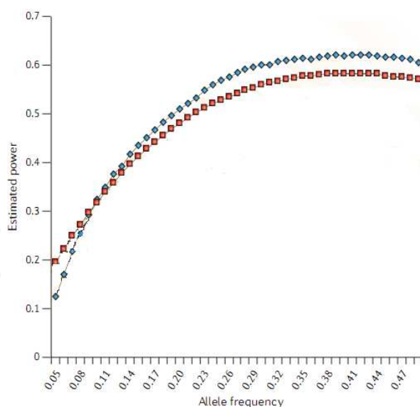
Fig. 1. The statistical power of GWA for blue case-control compared to red family trio (affected child and parents). This is modeled for a disease with 14% prevalence, similar to CVD in Australia. It should also be noted that a family design is more powerful for low frequency variants. Adapted from(Laird et al. 2006)
