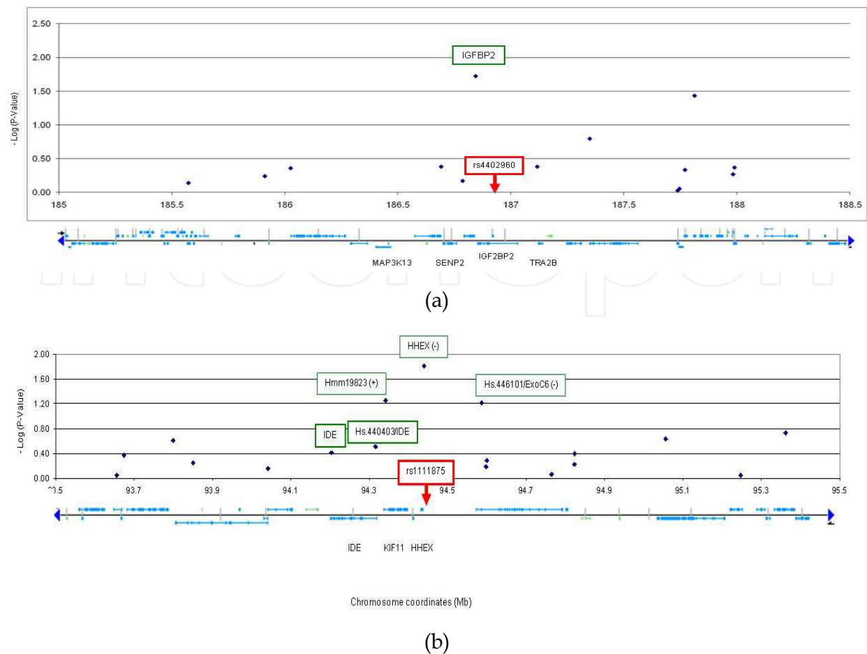
Fig. 5-a. Association of the rs4402960 SNP with the expression levels of genes within 5Mb of the SNP coordinate. Strong association of the IGF2BP2-residing SNP with IGF2BP2 is observed, suggesting that this locus mediates its effects through IGF2BP2 regulation of expression. 5-b. Association of the rs1111875 SNP with the expression levels of genes within 5Mb of the SNP coordinate. Strong association of the SNP with HHEX is observed, suggesting that this loci mediates its effects through HHEX regulation of expression. The intron/exon structure of the genes in this region is illustrated by the lines and blocks beneath the x-axis (thin line, intron; block, exon). The negative log of the P-value is plotted against the coordinates in megabase pairs (Mb). The methodology for this analysis was as reported for the FTO loci by Jowett and colleagues (Jowett et al., 2010).
