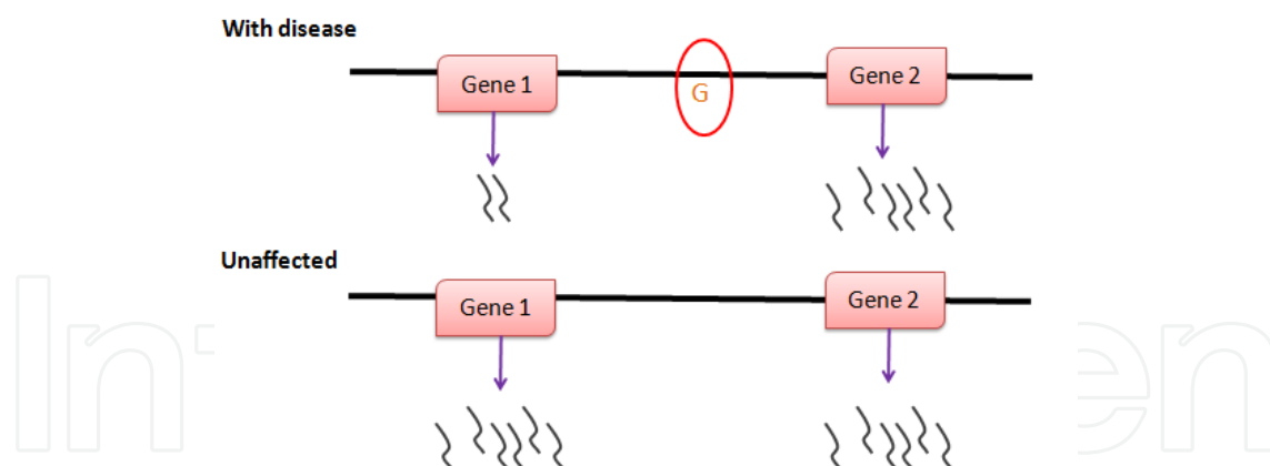
Fig. 4. GWA has found the circled SNP to be associated with a disease. It can be difficult though to assign this SNP to a candidate gene. Transcriptome analysis can make this easier by comparing the expression levels of flanking genes to each other, and between affected and unaffected individual. The decreased expression of gene 1 is associated with the disease, suggesting that gene 1 is the better candidate gene.
