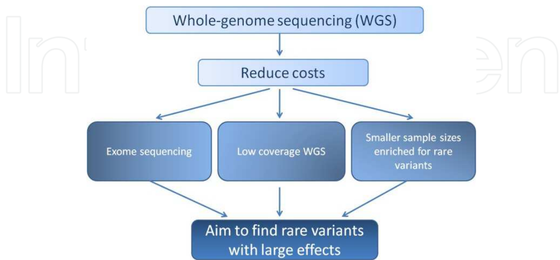
Fig. 6. Until WGS is affordable, alternatives such as exome sequencing, low-coverage WGS and smaller sample sizes reduce costs for a sequencing approach.
