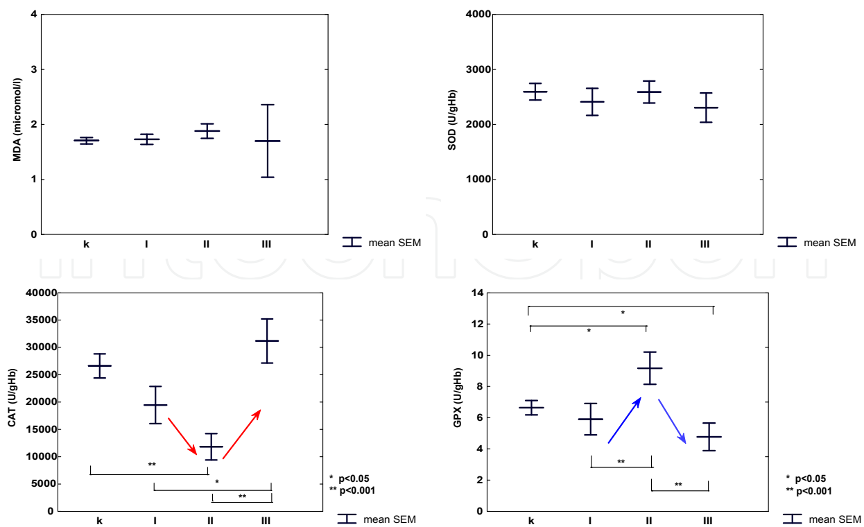
Fig. 5. Comparison of MDA levels in plasma and the activities of antioxidative enzymes superoxide dismutase (SOD) (U/ gHb), catalase (CAT) (U/ gHb), and glutathione peroxidase (GPX) (U/ gHb) in erythrocytes of control group and Hashimoto’s thyroiditis patients – euthyroid group (I), hypothyroid group (II) and group of patients treated with Levothyroxine (III). The results are expressed as mean ± S.E.
