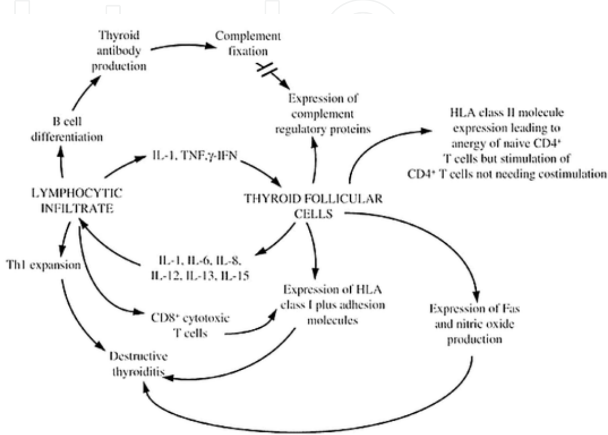
Fig. 1. Interaction between thyroid cells and the immune system via cytokines.
