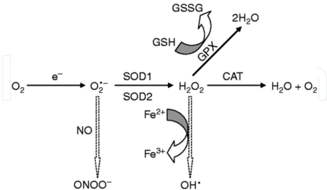
Fig. 4. Schematic representation of the pathways producing reactive oxygen species (ROS) and key cellular antioxidant enzymatic systems controlling ROS production.
