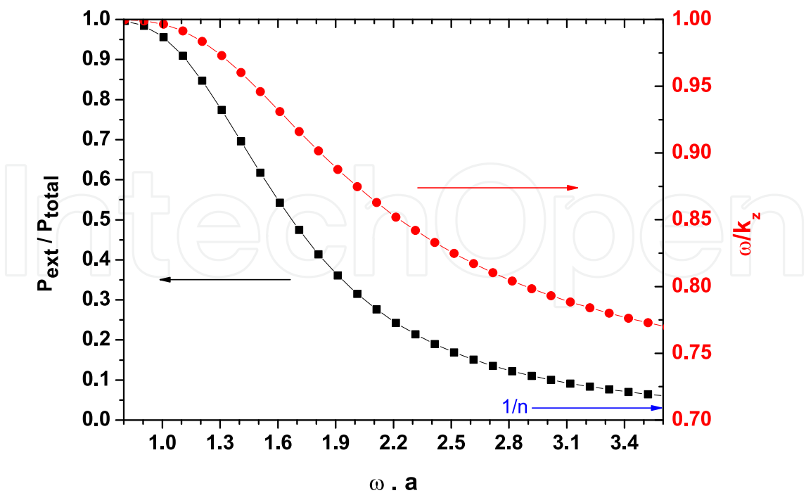
Fig. 2. Phase velocity v_{ph} = \omega / p (balls, right scale) and external fraction of the power (squares, left scale) for the HE_{11} mode.
