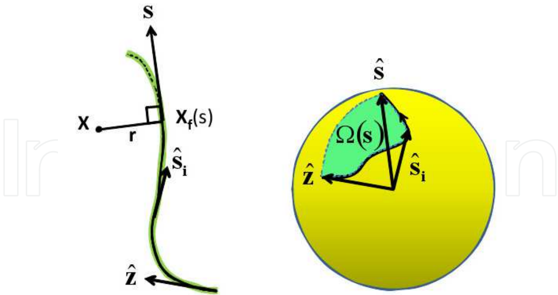
Fig. 3. Left: bent fiber and definition of X_f(s) and r . Right: curve drawn by the extremities of successive tangent vectors ( \hat{z} , \hat{s}_i , \hat{s} , ...) on the unit sphere and definition of the solid angle \Omega(s) . The dotted arc of circle represents the “most direct” rotation, \mathcal{R}(\hat{z} \rightarrow \hat{s}) , transforming \hat{z} into \hat{s} .
