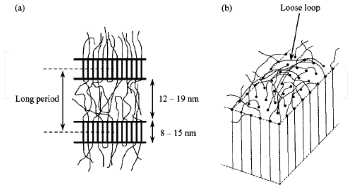
Fig. 4. Schematic illustrations of “switchboard-type” lamella models of fluorinated copolymers like an EFA (a) along the c -axis, and (b) in an a-b plane.
