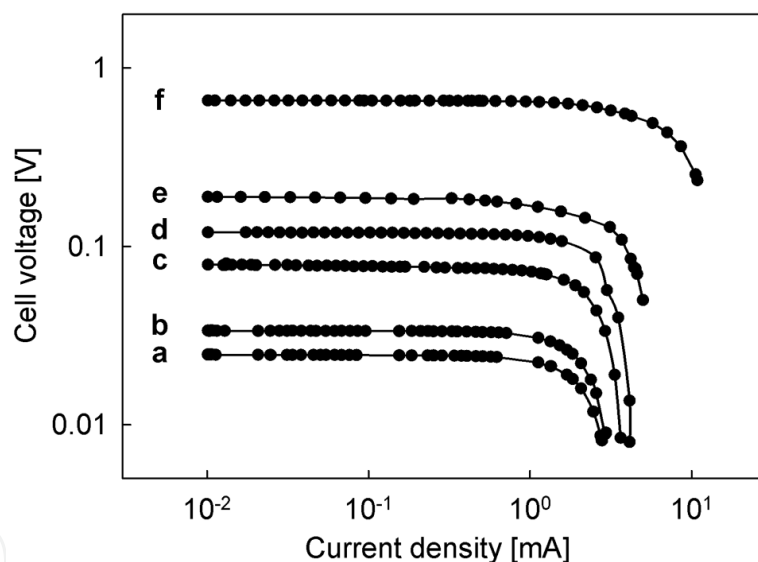
Fig. 13. Fuel cell characteristic for various cathode catalytic materials: (a) – CuO x ( t = 12 min); (b) – Co 3 O 4 ( t = 12 min); (c) – Co 3 O 4 +CuO x ( t = 12 min); (d) – Co 3 O 4 ( t = 60 min); (e) – Co 3 O 4 ( t = 80 min); (f) – Pt (Tyczkowski, 2011).
