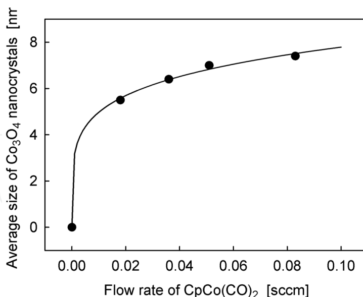
Fig. 12. Dependence of the average size of Co 3 O 4 nanocrystals on the flow rate of CpCo(CO) 2 vapor through the plasma reactor (Tyczkowski, 2011).
