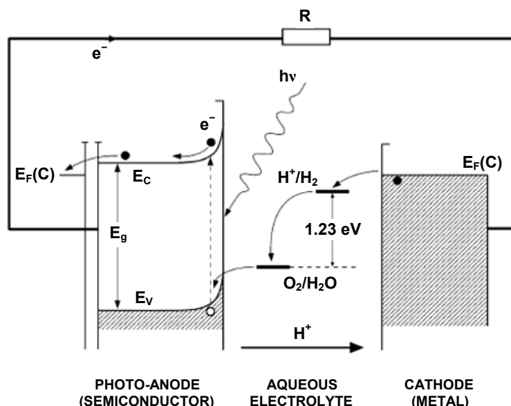
Fig. 7. Schematic representation of charge transfer within a photoelectrochemical cell involving a semiconducting photoanode and metal cathode (Nowotny et al., 2006).
