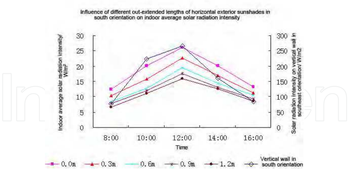
Fig. 9. Influence of horizontal exterior sunshade in south orientation on indoor average solar radiation
