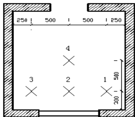
Fig. 7. Test points of indoor sola radiation intensity
