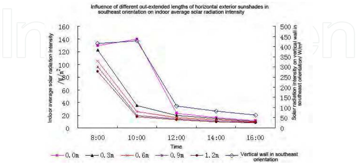
Fig. 8. Influence of horizontal exterior sunshade on indoor average solar radiation in southeast orientation
