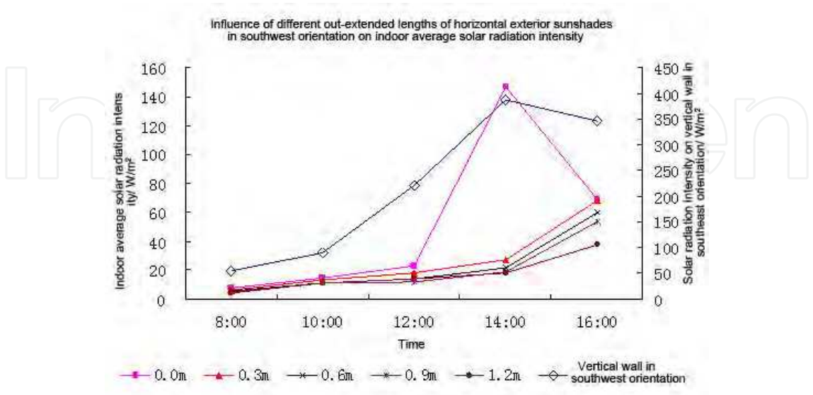
Fig. 10. Influence of horizontal exterior sunshade in southwest orientation on indoor average solar radiation
