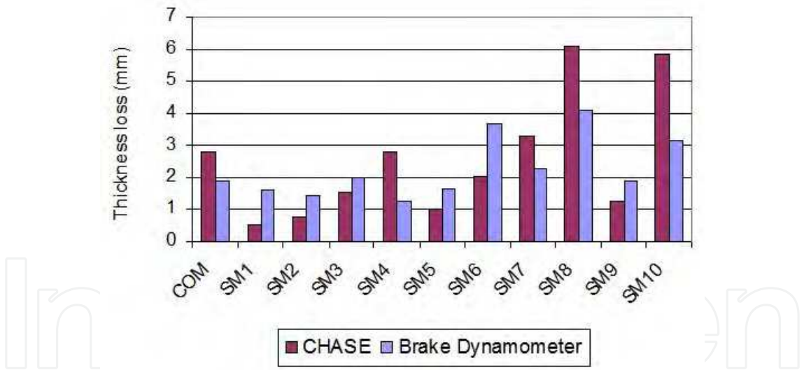
Fig. 12. Bar chart of thickness loss during CHASE and dynamometer test.
