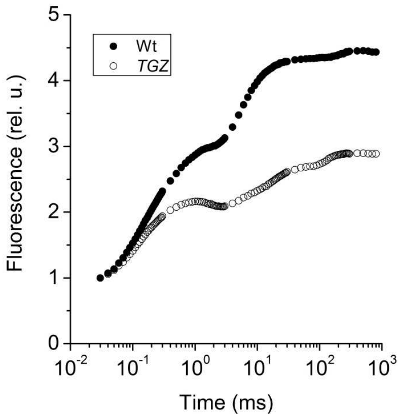
Fig. 4. Fluorescence induction curves of Nicotiana tabacum Wt and tobacco over-expressing tgz from maize (TGZ). Samples were dark adapted for 20 min and were illuminated with 3000 μmol [photons] m -2 s -1 . The time axis is semi-logarithmic for clarity and data are normalized to Fo.
