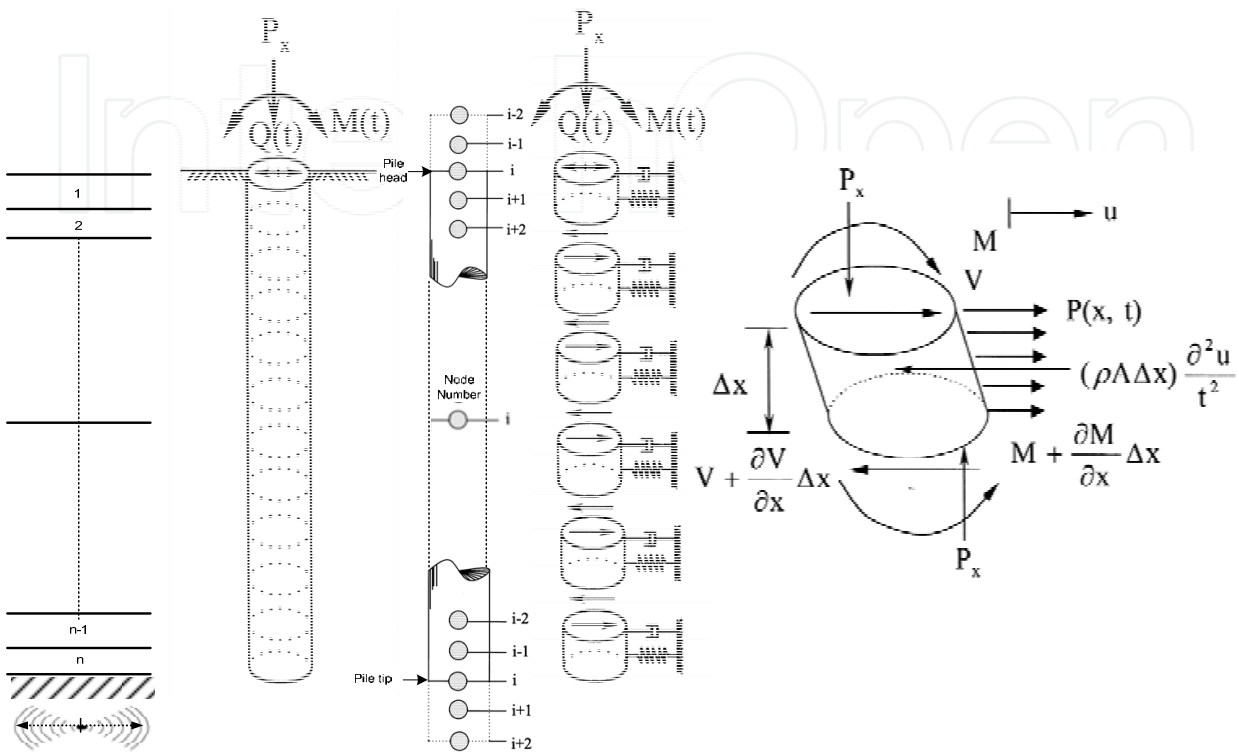
Fig. 1. Discrete system of the single pile
