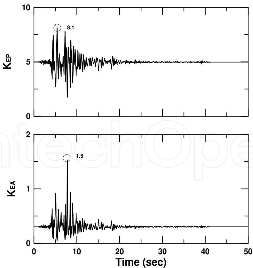
Fig. 16. Dynamic coefficients of earth pressure
