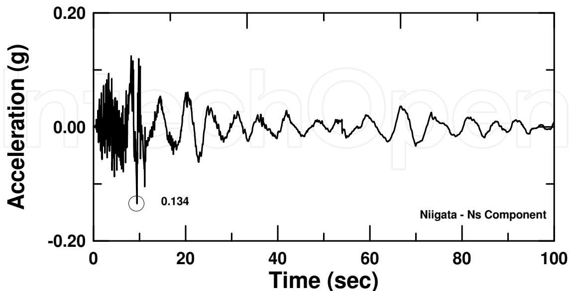
Fig. 10. Time history of Niigata Earthquake (NS Component)
