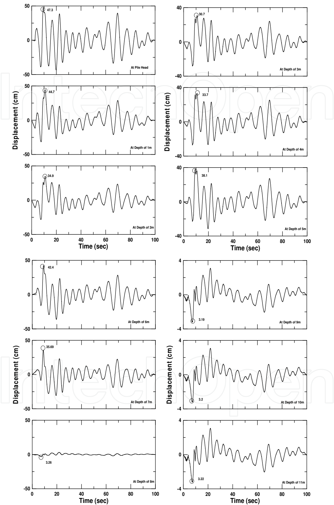
Fig. 12. Time histories of ground motions at different depths
