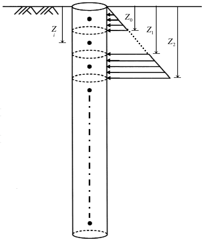
Fig. 6. Distribution of earth pressure along a pile
