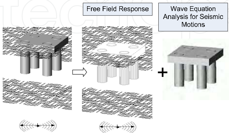
Fig. 2. Superposition of the free-field analysis and WEA
