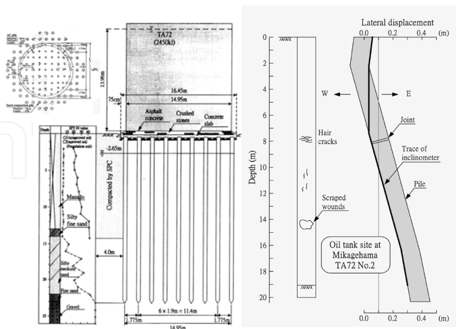
Fig. 15. Cross sectional view of Tank TA 72 and its foundation (from Ishihara and Cubrinovski, 2004)
