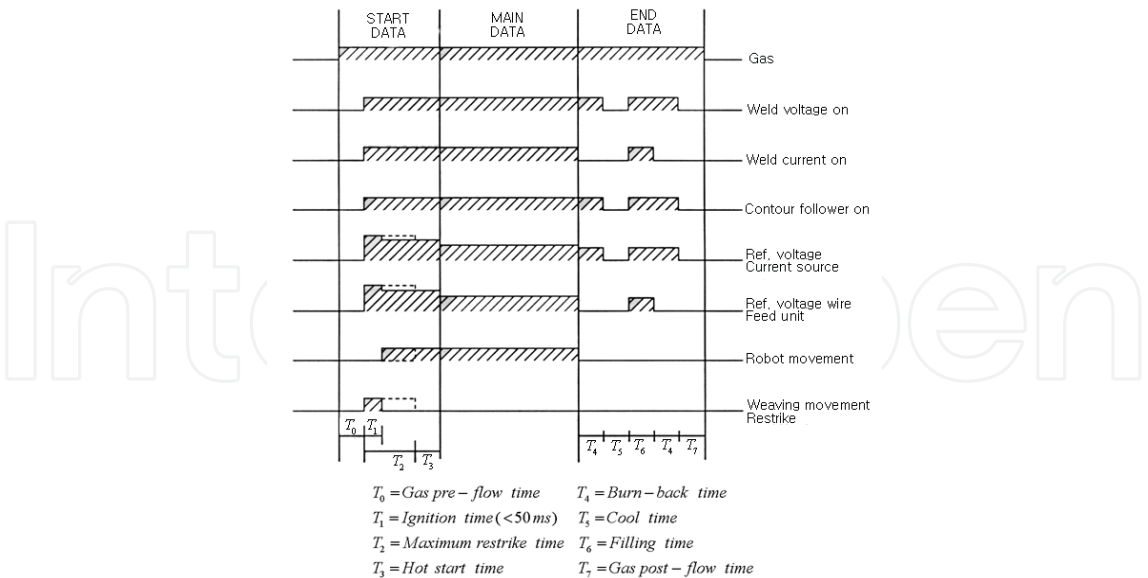
Fig. 14. An Example of Welding Data.
