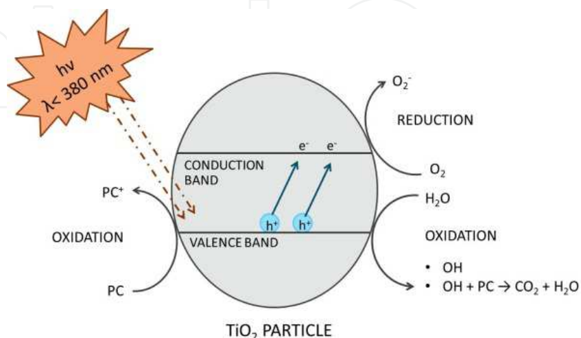
Fig. 3. Basic photocatalytic process involving TiO 2 particle
