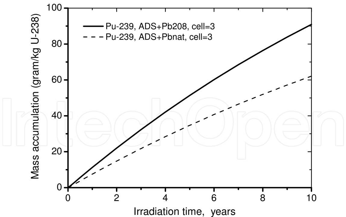
Fig. 6. Mass accumulation of Pu-239 in the ADS 80 MW subcritical blanket in inserting 1 kg of U-238. in the cell 3, near the blanket’s far margin. The solid curve corresponds to the case, when the blanket is cooled with lead-208, the dash curve – to the case, when the blanket is cooled with lead natural.
