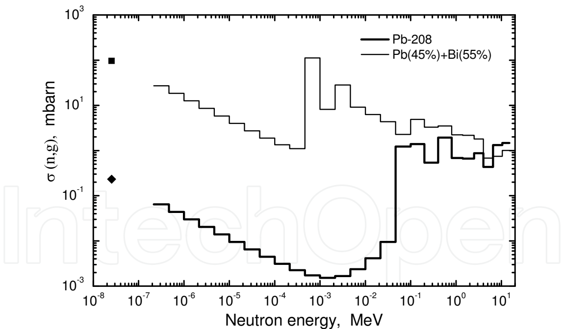
Fig. 2. Microscopic cross sections of radiation neutron capture s(n,g) by stable lead-208 isotope and by the eutectic Pb-nat(45%) – Bi (55%) taken from the ENDF/B-VII.0 library. Cross sections are represented in the ABBN-93 system of 28 neutron energy groups.
