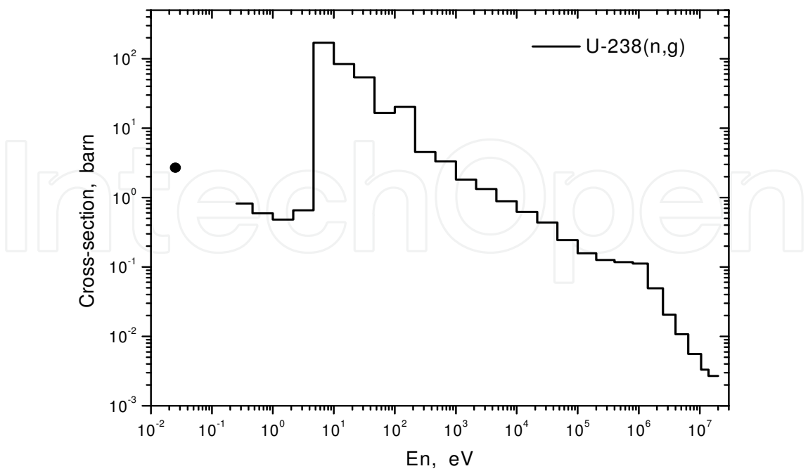
Fig. 5. Microscopic cross sections of radiation neutron capture by uranium-238 taken from ENDF/B-VII.0 library.
