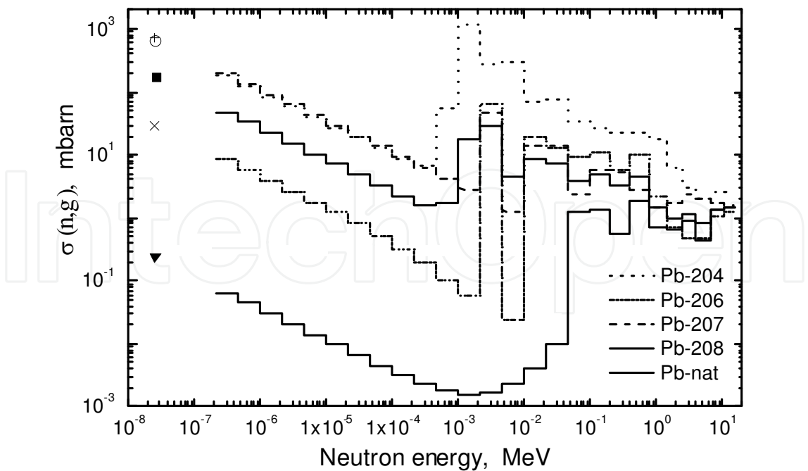
Fig. 1. Microscopic cross sections of radiation neutron capture s(n,g) by stable lead isotopes and by natural mix of lead isotopes taken from the ENDF/B-VII.0 library. Cross sections are represented in the ABBN-93 system of 28 neutron energy groups.
