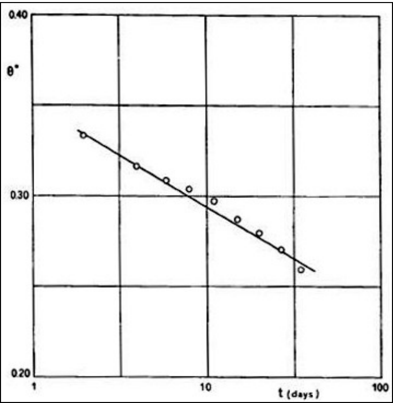
Fig. 19. Calculated curve (solid line) obtained by regression of equation 27 on measured (symbols) of water content \theta^* at depth z=75 cm
