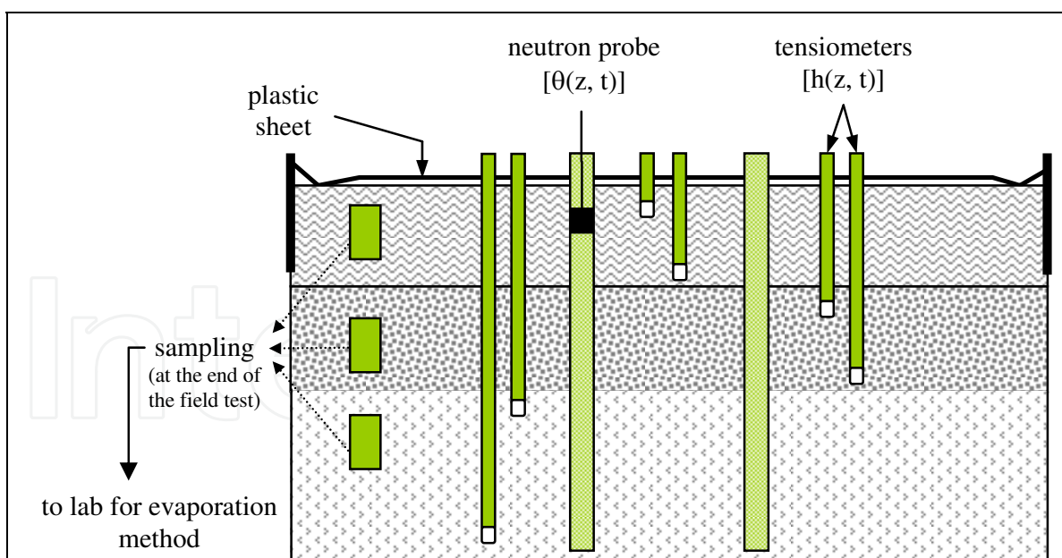
Fig. 15. Schematic of internal drainage setup
