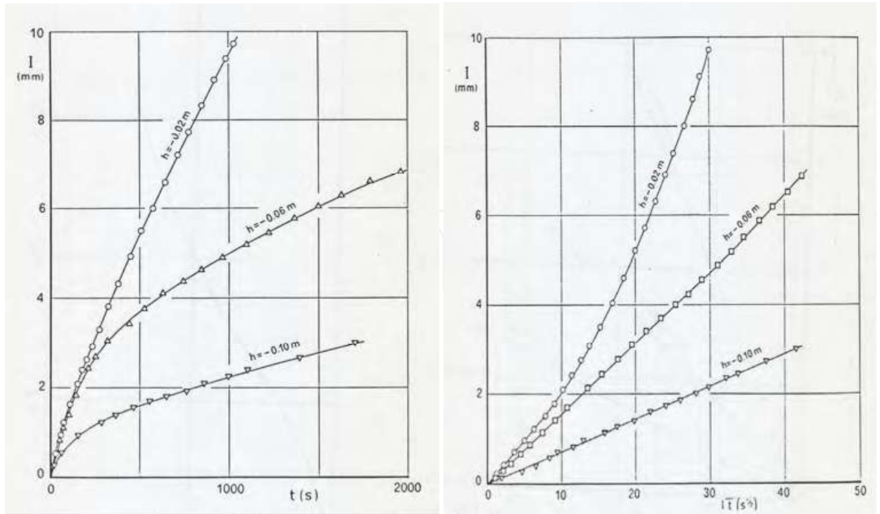
Fig. 24. a. In situ cumulative infiltration over time and b. over square root of time during 3D flow from disk permeameter for three water supply potentials
