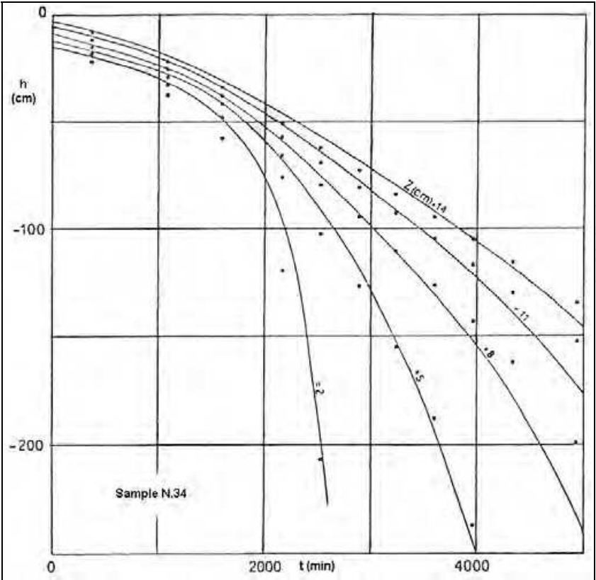
Fig. 3. Measured (circles) and calculated (solid lines) h(t) data for different depths of sample 34
