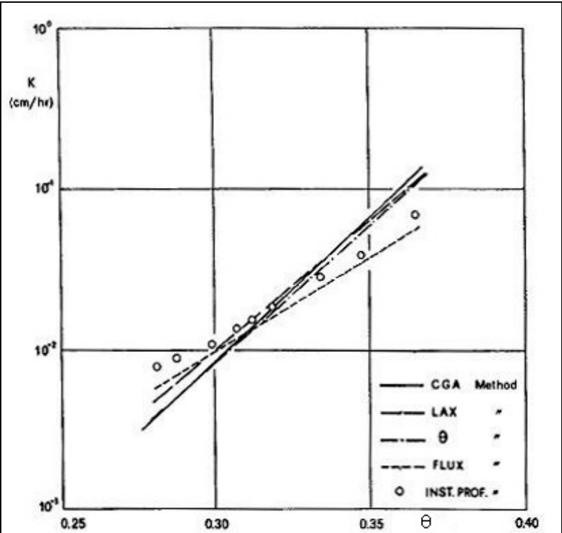
Fig. 20. Comparison between K(\theta) calculated (solid line) and measured (symbols) at z=75\text{ cm}
