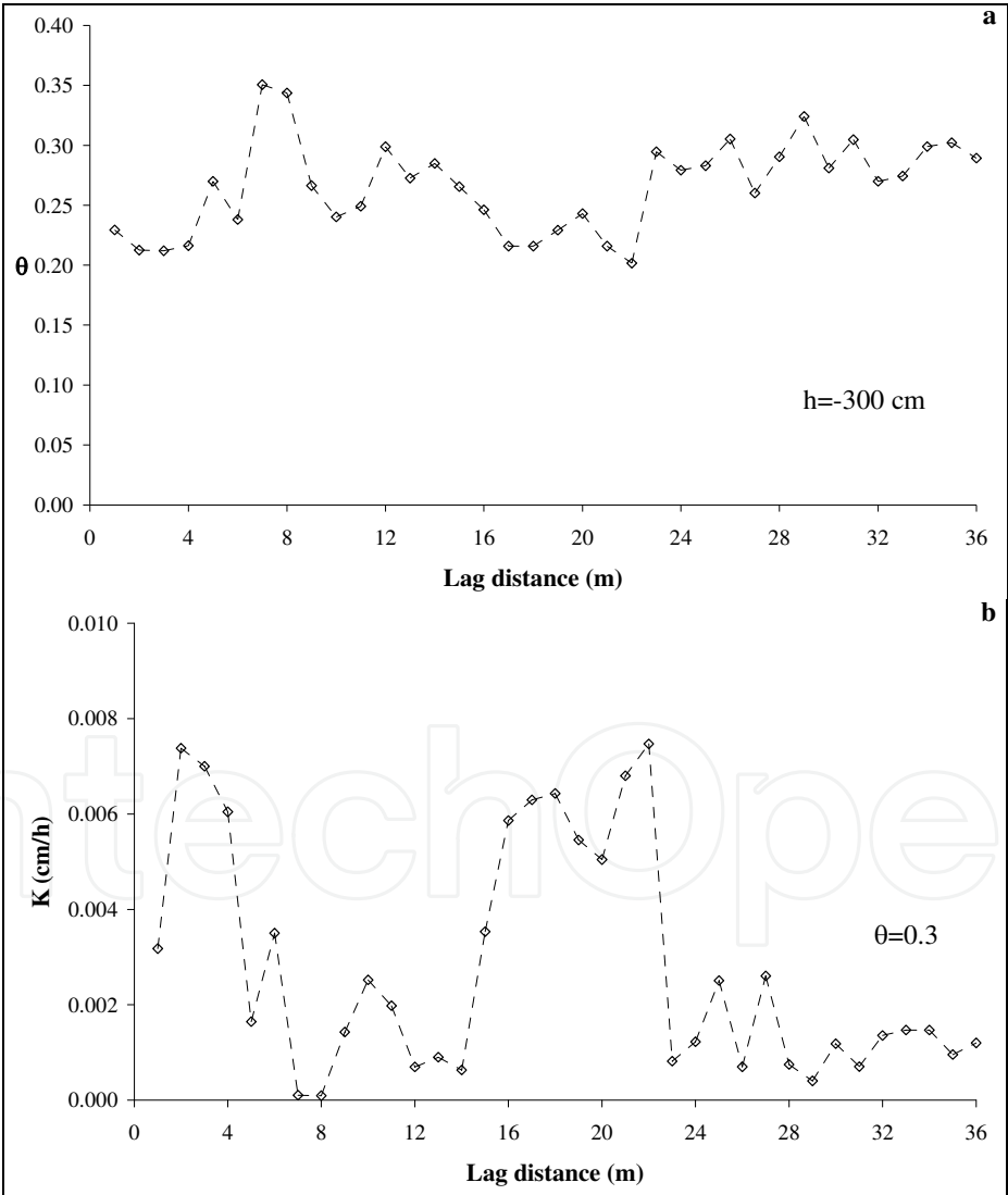
Fig. 29. a. Series of \theta_i values, i=1, 2, \dots, 36 obtained from water content measurement for h=-300 cm; b. Series of K_i values, i=1, 2, \dots, 36 obtained from estimation of hydraulic conductivity for \theta=0.300
