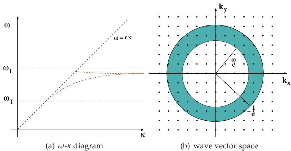
Fig. 4. Sketch of the surface phonon polariton modes for a given distance d . relation (Kliewer and Fuchs (1974))
