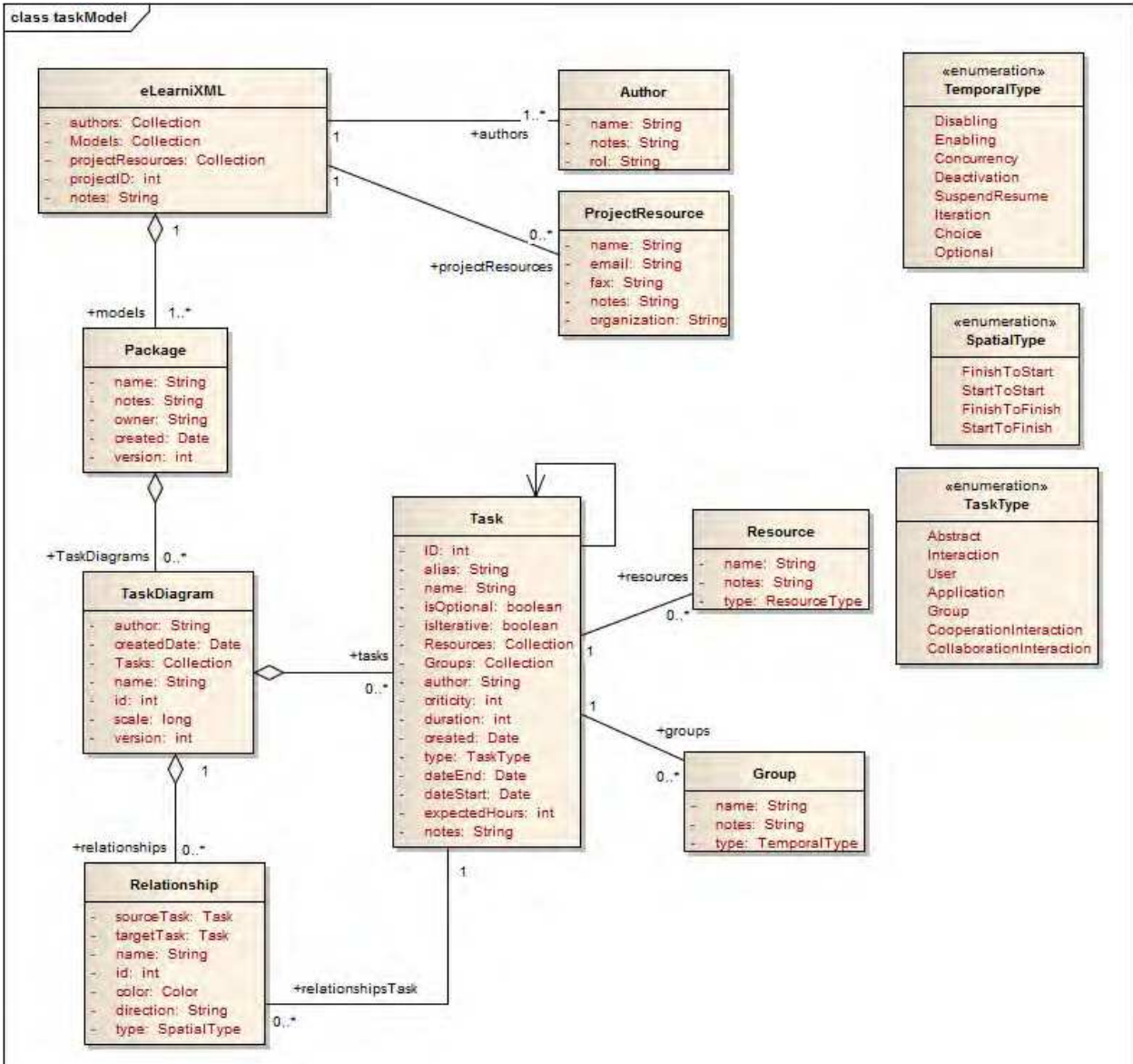
Fig. 13. ELearnXML task model.
