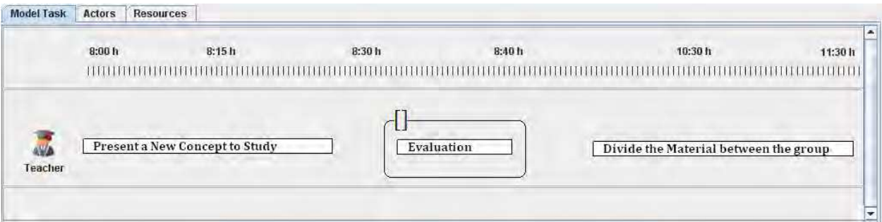
Fig. 11. Choice temporal operator presented by eLearnXML notation.
