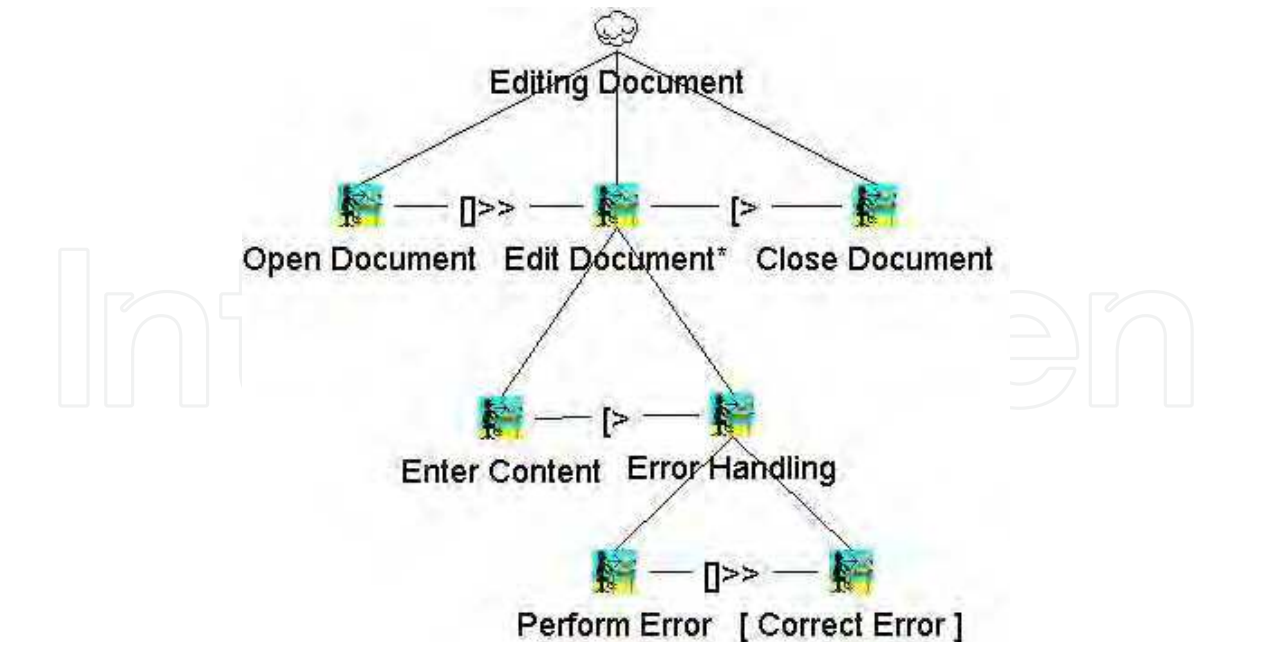
Fig. 3. A task model sample with Concur Task Tree notation.
