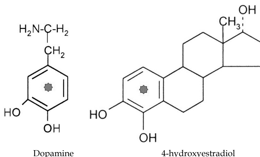
Fig. 8. The dopamine structure and the 4-hydroxyestradiol structure.
