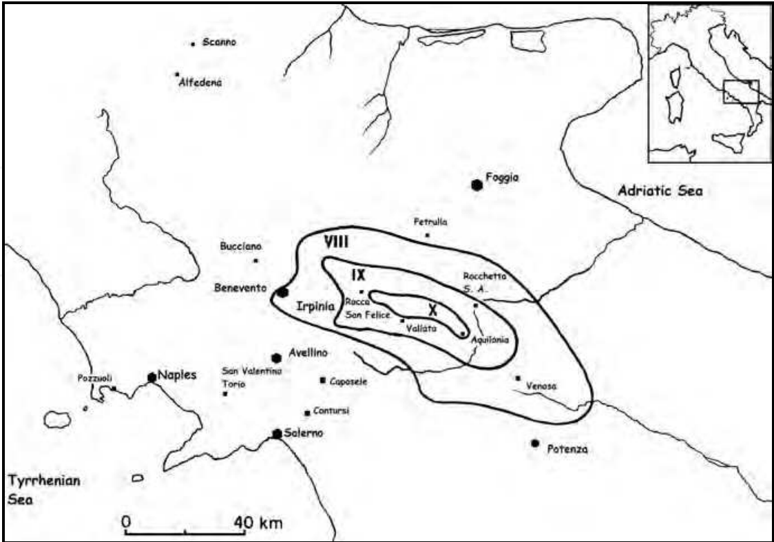
Fig. 2. (a) Iseismal map for the 1930 earthquake
