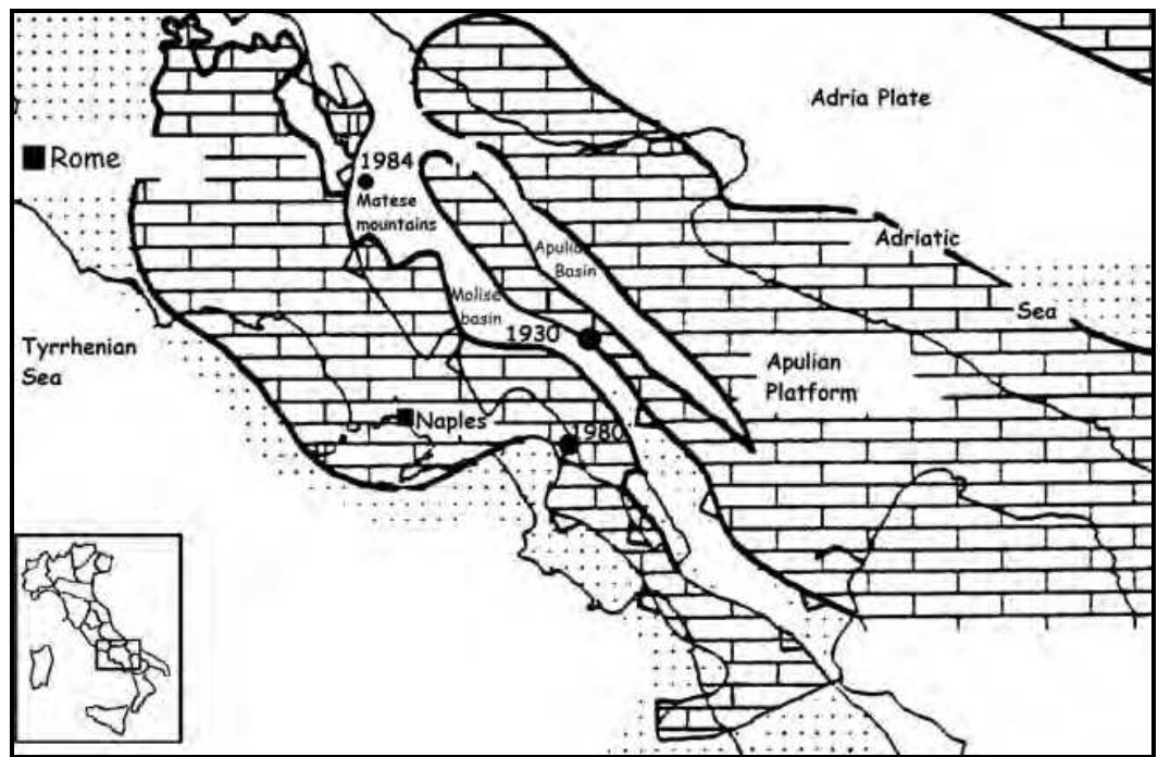
Fig. 1. (a) Sketch map of the Southern Apennines.
