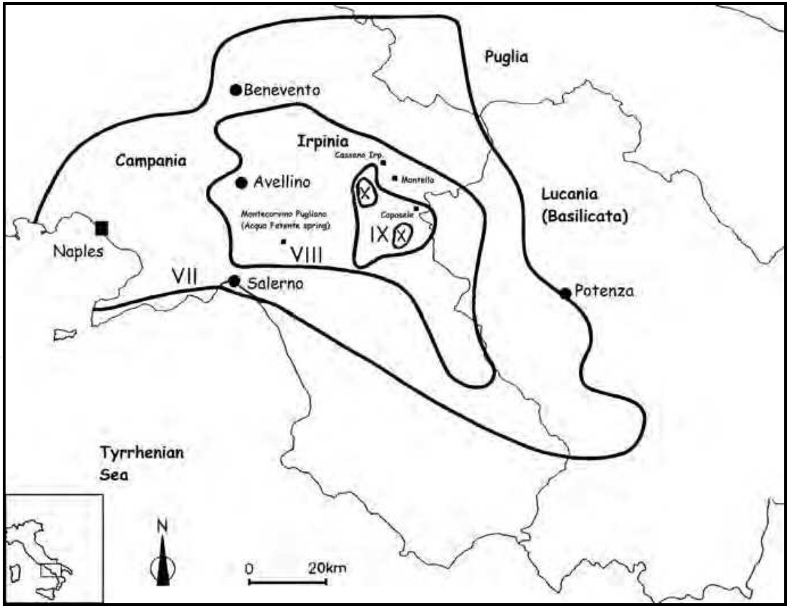
Fig. 2. (b) Iseismal map for the 1980 earthquake
