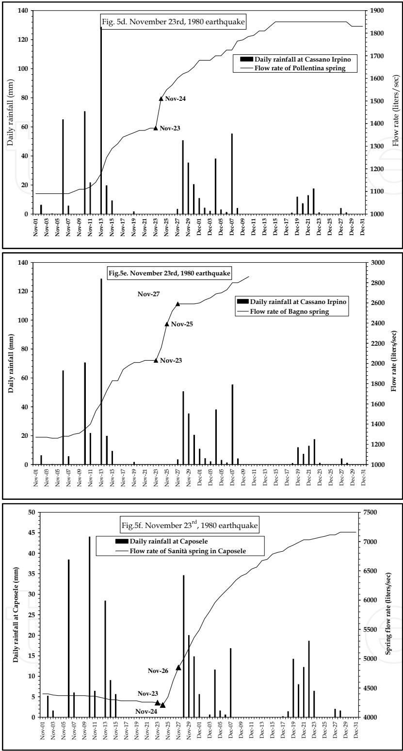
Fig. 5. Acqua Fetente spring (a); Zittola river at Montenero (b); Streamflow level of Calore Irpino at Montella (c); Cassano Irpino springs: Pollentina (d) and Bagno (e); Sanità spring at Caposele (f).
