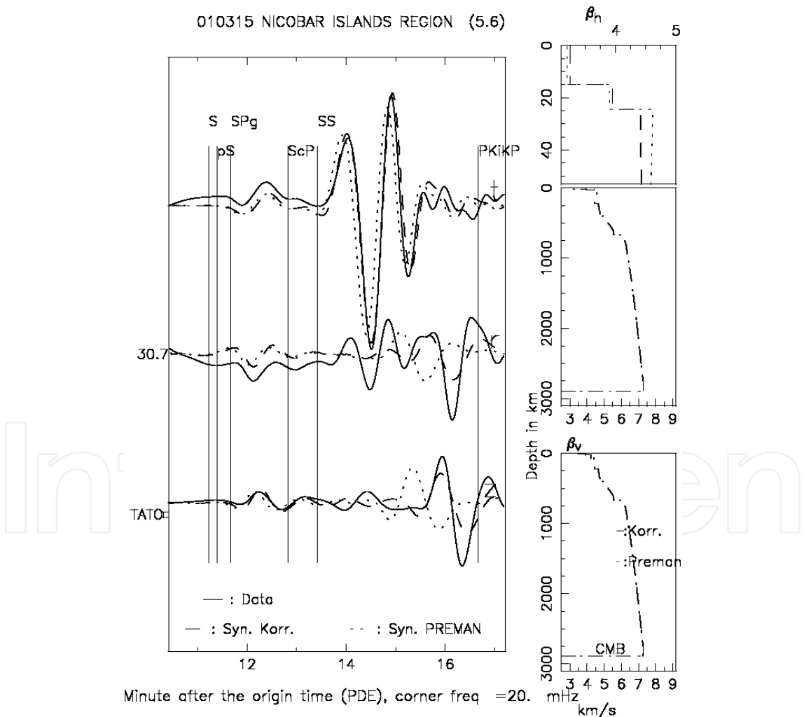
Fig. 3. The seismogram fitting of Nicobar B031501B earthquake in TATO.
