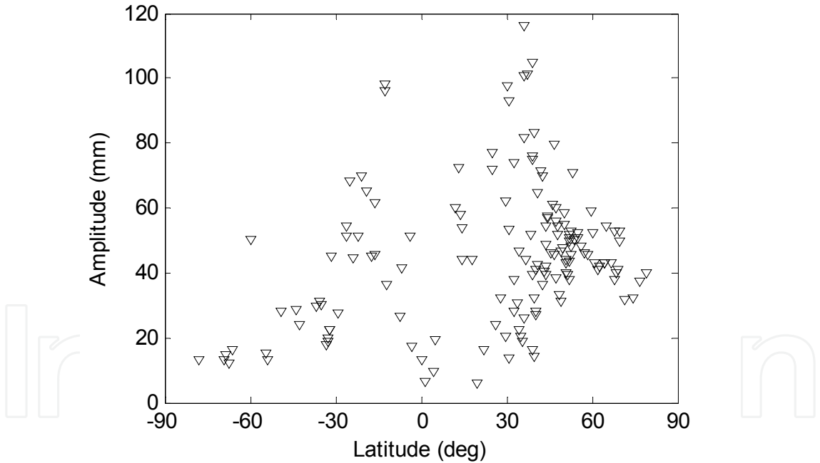
Fig. 6. Distribution of annual ZTD variation amplitude with the latitude
