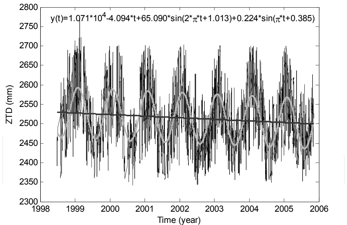
Fig. 2. ZTD time series at TOW2 station, Australia. The solid line is the fitting results, consisting of a linear decrease and seasonal components
