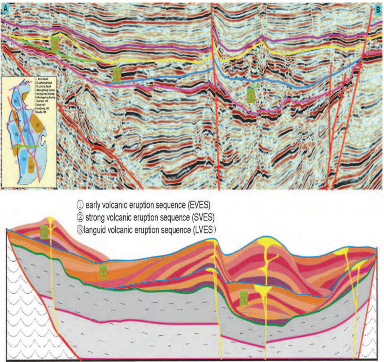
Fig. 11. The map of volcanic sequence division
