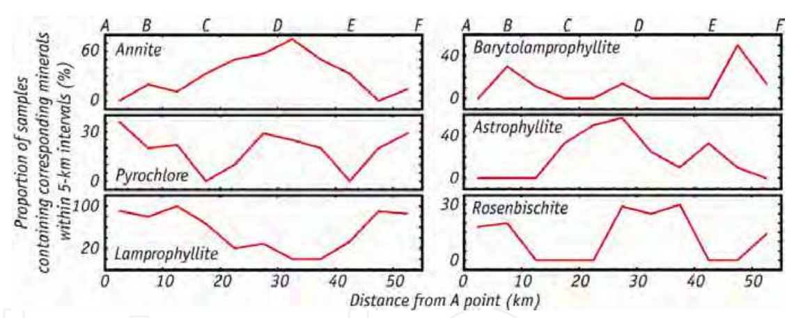
Fig. 7. Variation of accessory mineral contents along the A-B-C-D-E-F profile.
