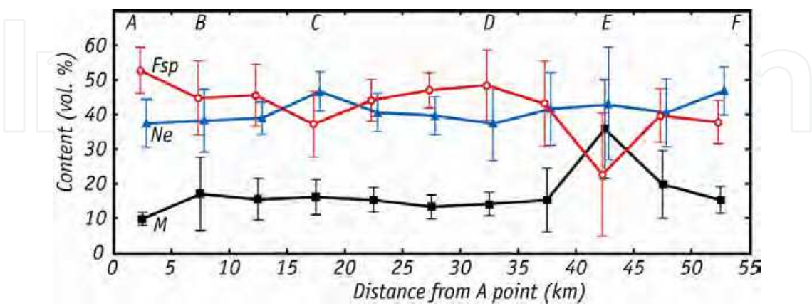
Fig. 6. Variation of alkaline feldspar (Fsp), nepheline (Ne) and dark coloured minerals (M) contents along the A-B-C-D-E-F profile (mean plus-minus standard deviation).
