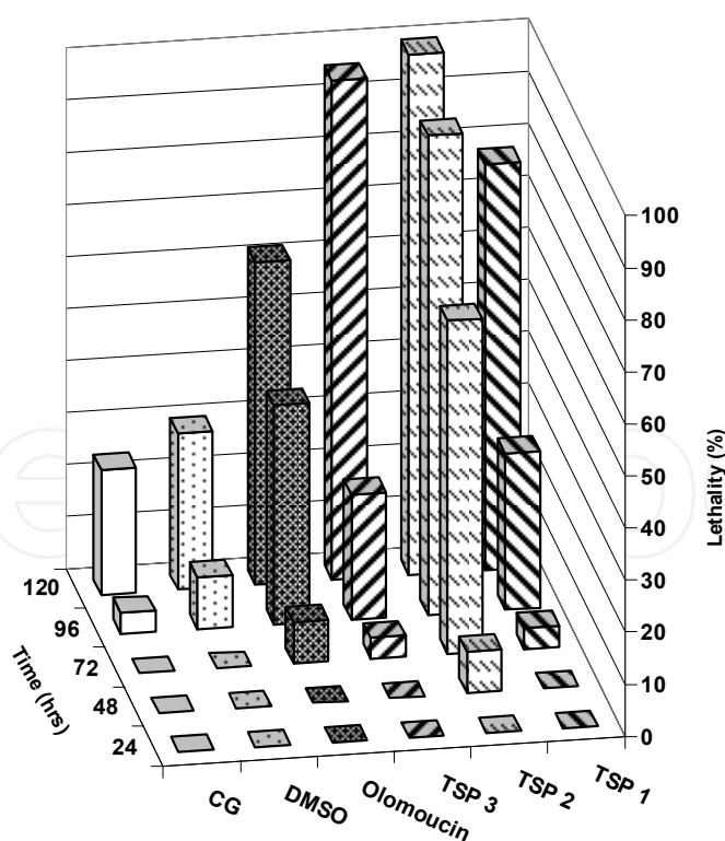
Fig. 4. Comparison of effects of newly synthesised CDKI (TSP 1, TSP 2, and TSP 3) with effects of olomoucine ( 100 \text{ mg.L}^{-1} ) on lethality of A. franciscana . All substances were dissolved in dimethylsulfoxide (DMSO, 15 \text{ g.L}^{-1} ); CG – control group without DMSO.
