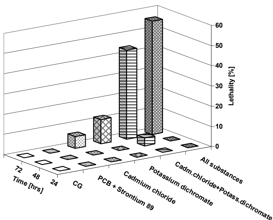
Fig. 2. Effect of simultaneous treatment with strontium 89 [33 kBq.L -1 ], PCB - delor 103 [4.5 ng.L -1 ], cadmium chloride (CdCl 2 · 2H 2 O) [Cadm.chloride; 20 mg.L -1 ], and potassium dichromate [Potass.dichromate; 5 mg.L -1 ] on lethality of A. franciscana ; CG - control group (no agents).
