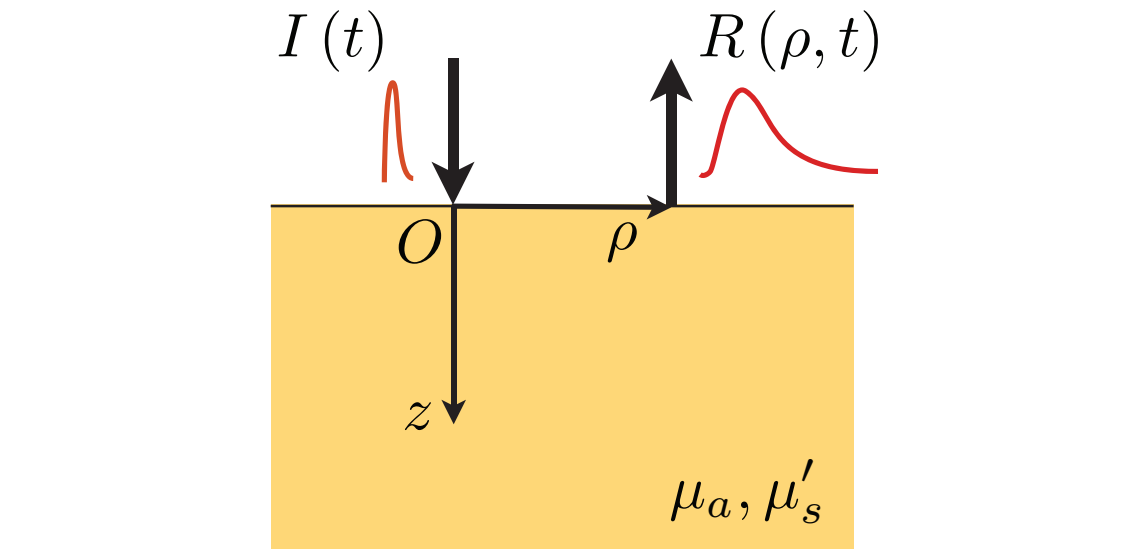
Fig. 5. Scheme of reflection geometry TD-NIRS measurement. Injected light travels in the medium and part of it can be collected by a detector at a source-detector distance \rho . Knowing the temporal shape of the injected light I(t) , the temporal shape of the collected light R(\rho, t) depends on \mu_a and \mu'_s .
