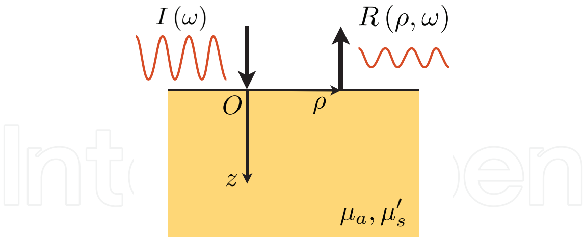
Fig. 4. Scheme of reflection geometry FD-NIRS measurement. Intensity modulated light I(\omega) travels in the medium and part of it can be collected by a detector at a source-detector distance \rho . Amplitude and phase of the collected light R(\rho, \omega) depend on \mu_a and \mu'_s .
