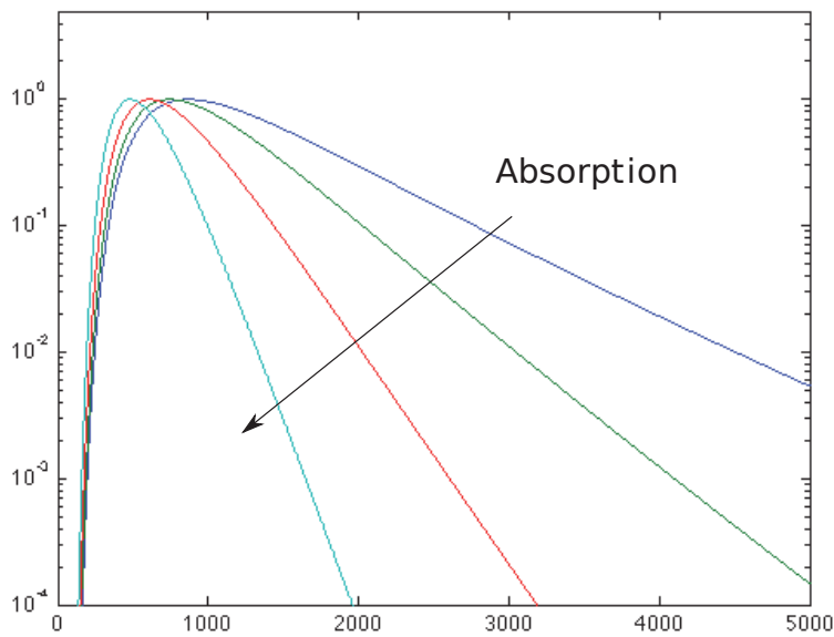
(b) Dependence from absorption ( \mu_a = 0.04, 0.08, 0.16, 0.32 cm -1 , \mu'_s = 20 cm -1 ).
