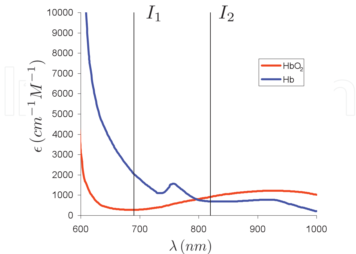
Fig. 1. The absorption spectrum, that is the molar extinction coefficient vs. the wavelength, of the oxygenated (red) and deoxygenated (blue) states of the hemoglobin. I_1 and I_2 are the chosen wavelengths for Near InfraRed Spectroscopy measurements.
