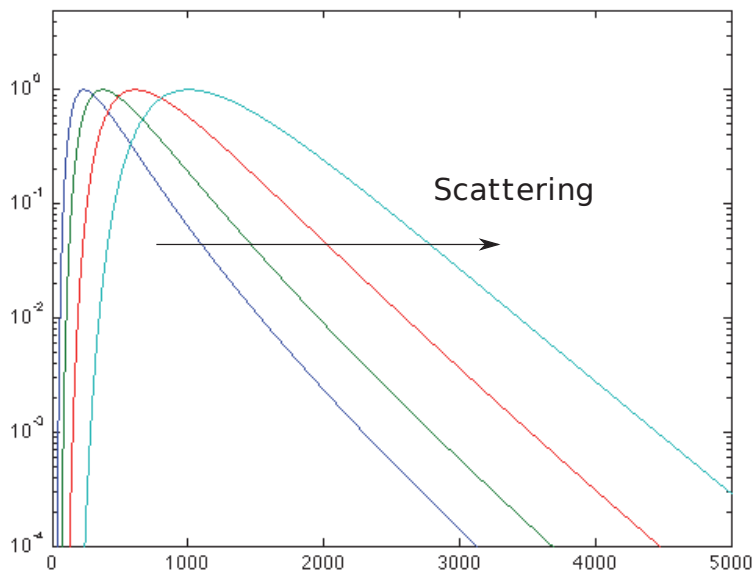
(a) Dependence from scattering ( \mu_a = 0.09 cm -1 , \mu'_s = 4, 8, 16, 32 cm -1 ).
