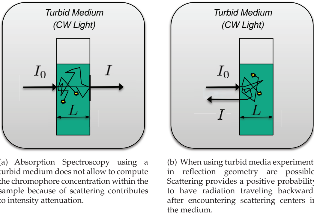
Fig. 3. Absorption spectroscopy in turbid medium in trasmission geometry (Fig. 3(a)) and reflection geometry (Fig. 3(b)).
