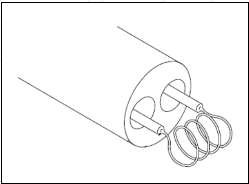
Fig. 3. The stress relieving coil of Au/Pt thermocouple.
