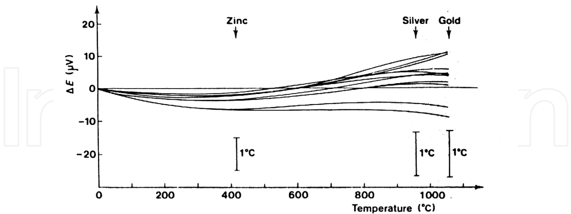
Fig. 7. Difference curves between the IEC Standard Reference Table and the emfs of a series of Pt-13%Rh/Pt thermocouples.
