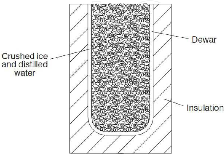
Fig. 4. Ice bath for reference junction
