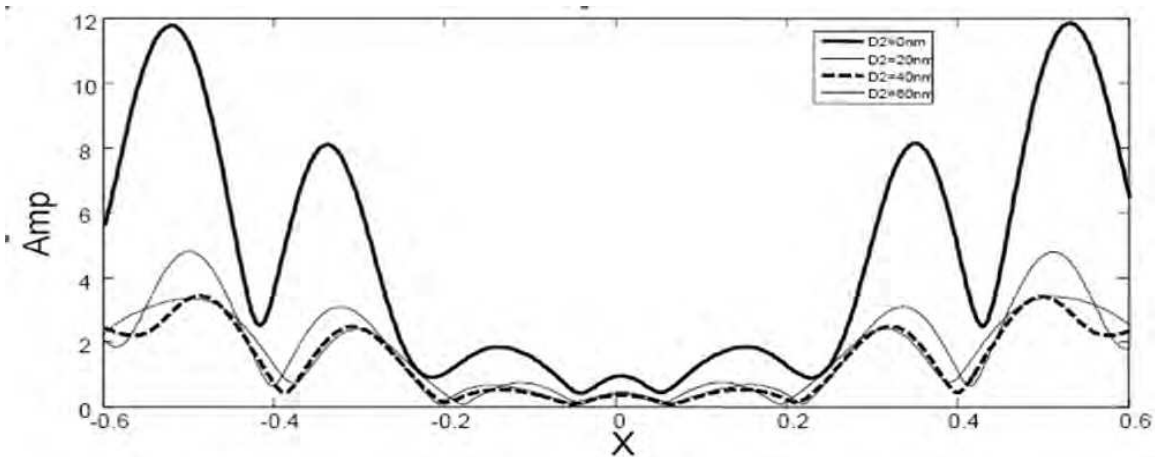
Fig. 4. The distribution of optical field in the 10 nm cross-section of photoresist when D1=40\text{ nm} .
