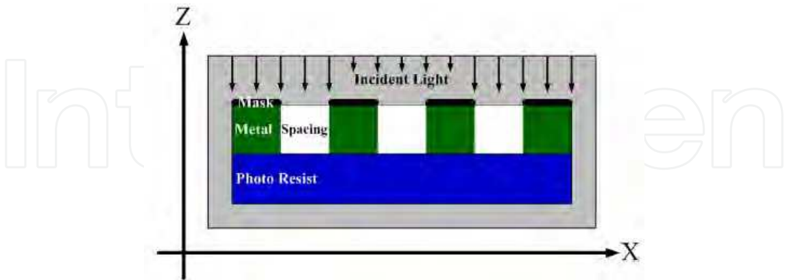
Fig. 12. Sketch of subwavelength optical lithography method.
