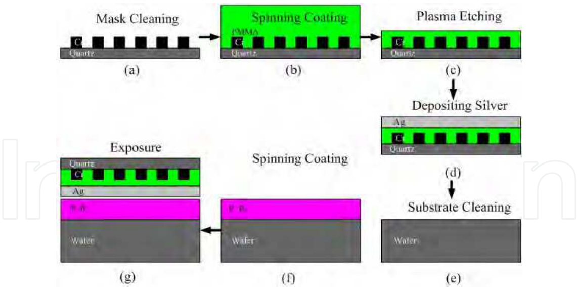
Fig. 10. The special process for the nanolithography.
