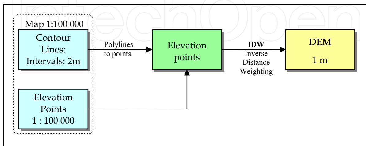
Fig. 3. The flowchart of Digital Elevation Model Generation procedure.
