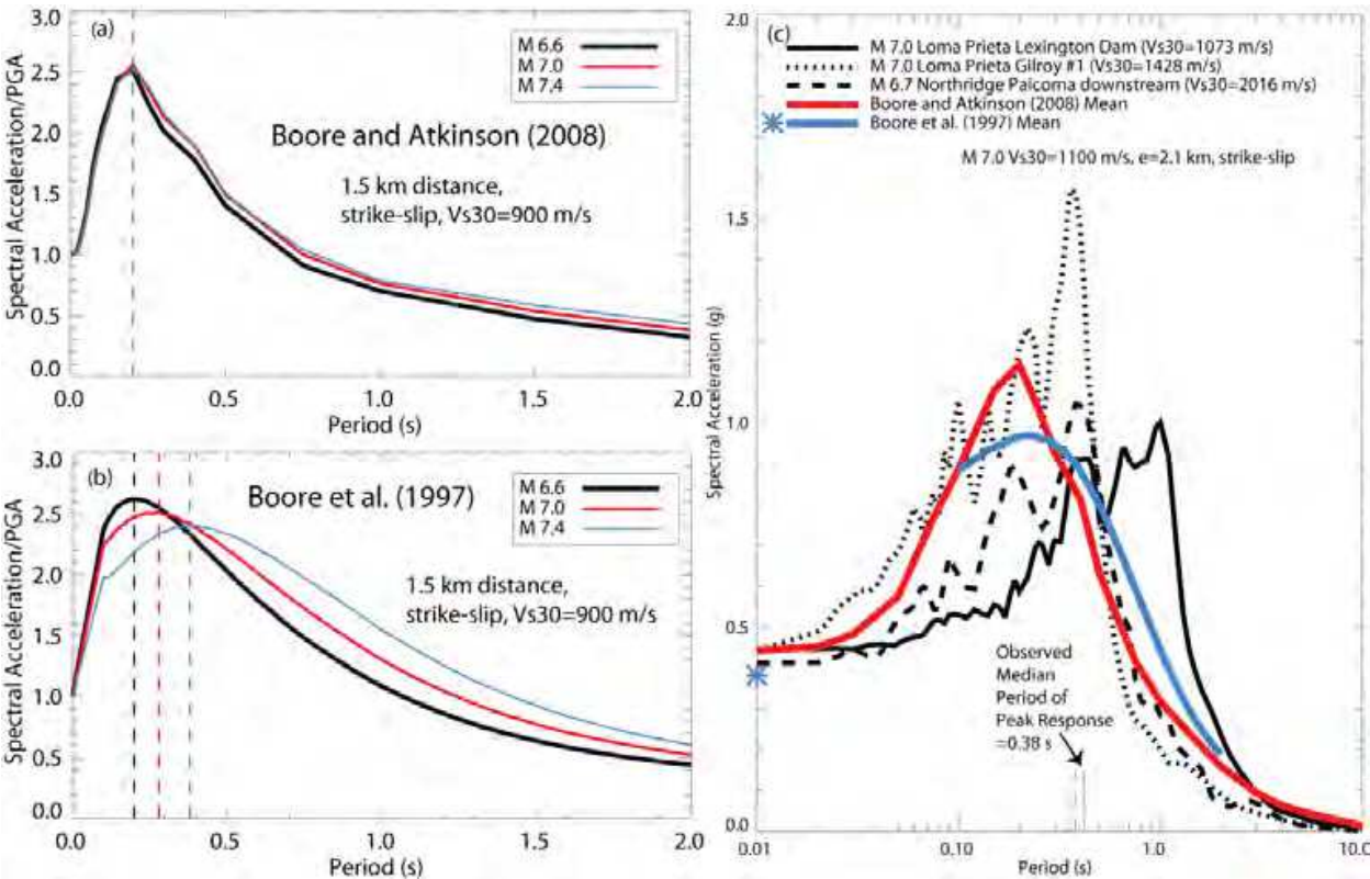
Fig. 5.3. Boore and Atkinson (2008) (a) and Boore et al. (1997) (b) response spectra normalized by peak ground acceleration for Vs30 =900 m/s. The geometric mean spectral accelerations from the three observed Vs30 > 900 m/s ground motions in Table 6 is compared to the mean Boore and Atkinson (2008) and Boore et al. (1997) estimates in (c).
