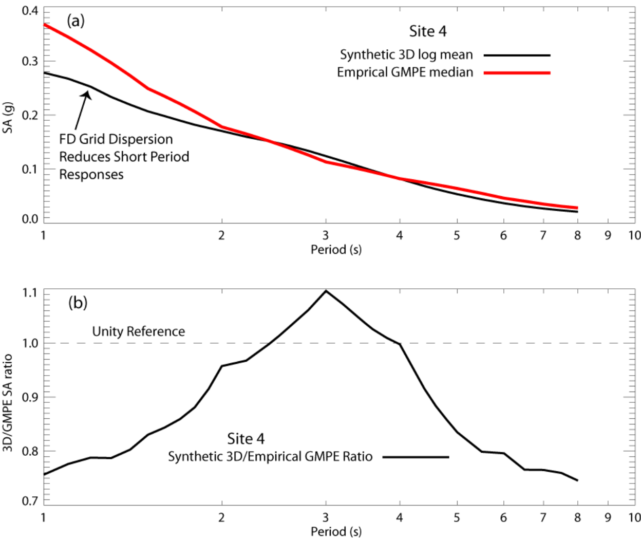
Fig. 5.7. Site 4 3D synthetic and NGA GMPE mean response spectra (a) and the 3D/NGA GMPE ratio (b).
