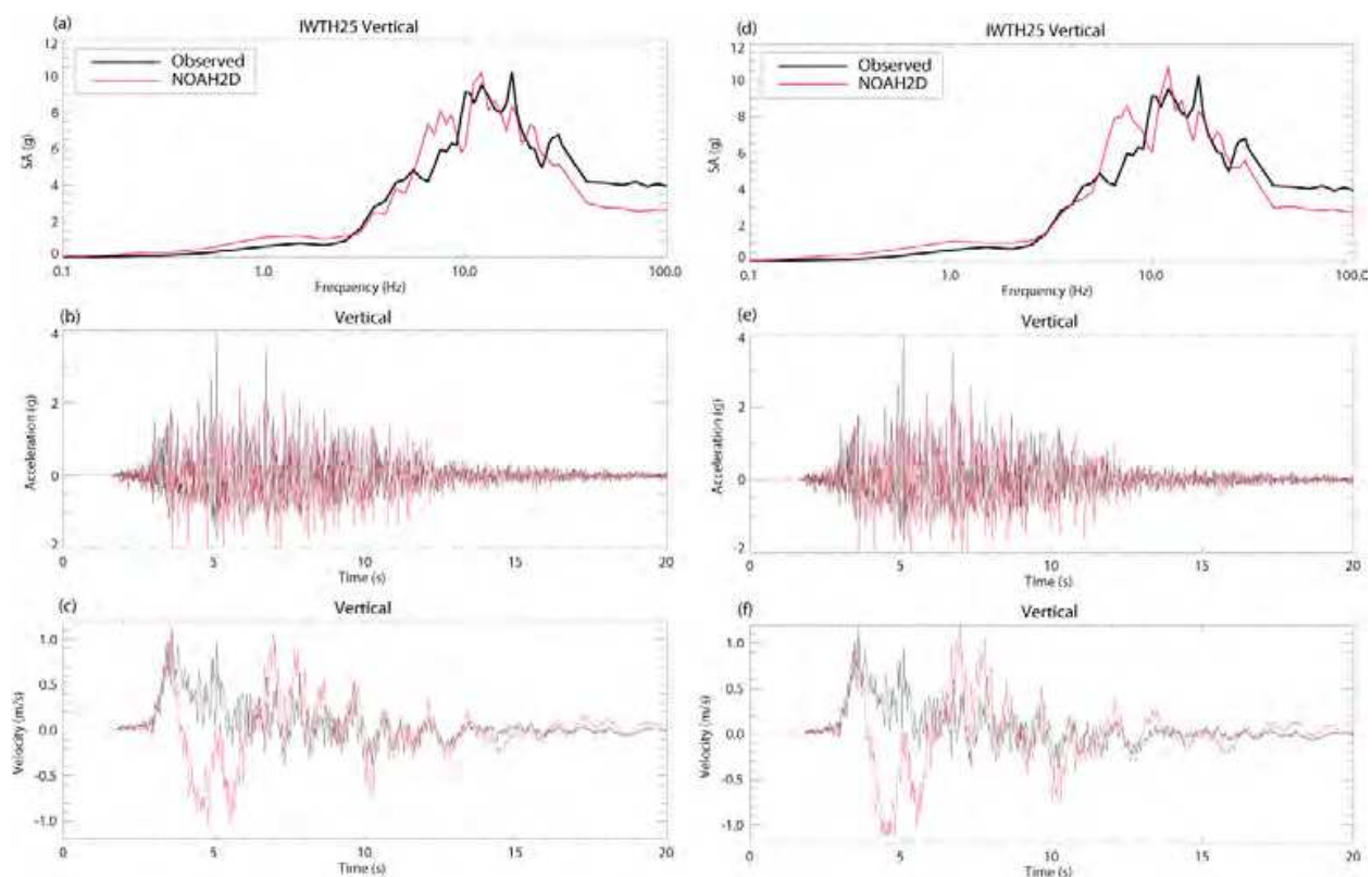
Fig. 4.9. Observed and simulated surface Iwth25 vertical response spectra (a,d), and acceleration (b,e), and velocity (c,f) time histories using the north-vertical (a-c) and east-vertical (d-f) components.
