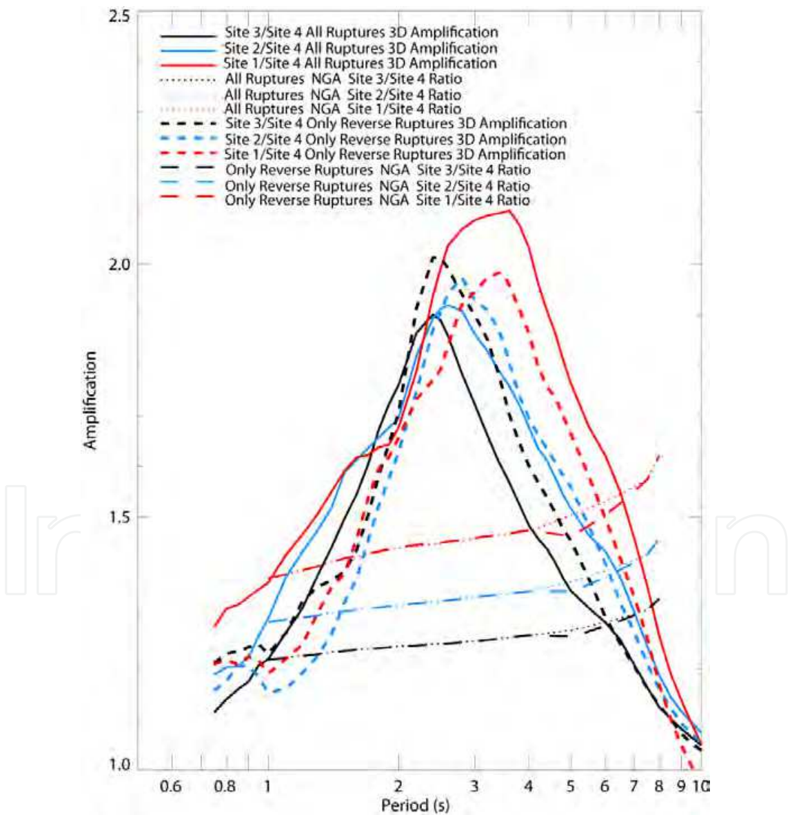
Fig. 5.8. Mean and reverse-rupture only residual 3D basin amplifications for sites 1-3 relative to reference site 4 with NGA differential site amplitude correction functions.
