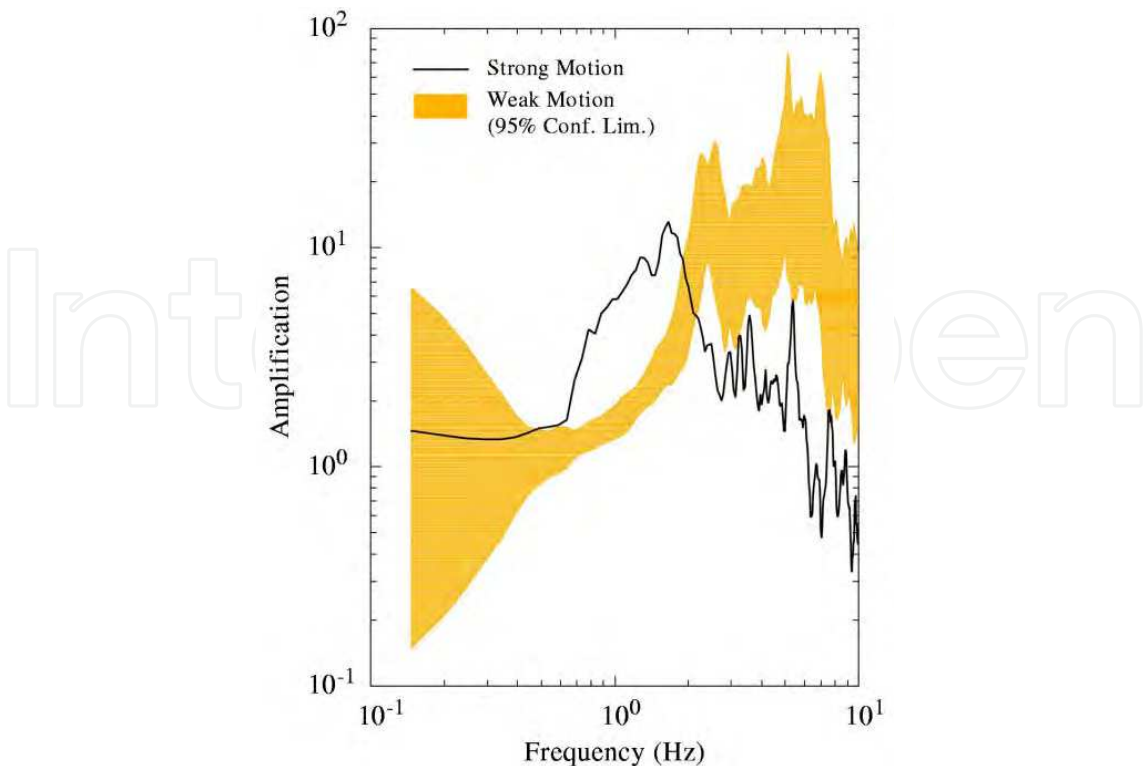
Fig. 4.2. Borehole transfer functions computed at KiK-net station TTRH02 in Japan. The orange shaded area represents the 95% confident limits of the transfer function using weak-motion events ( PGA < 10\text{cm/s}^2 ). The solid line is the transfer function computed using the October 2000 Tottori mainshock data.
