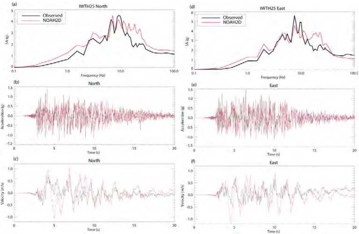
Fig. 4.8. Observed and simulated surface ITWH25 horizontal response spectra (a,d), and acceleration (b,e), and velocity (c,f) time histories for the north (a-c) and east (d-f) components.
