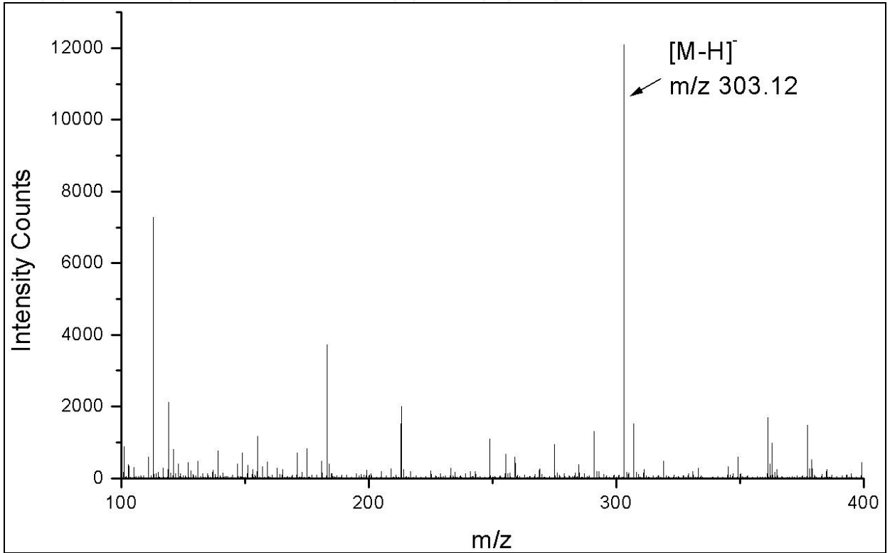
Fig. 7. Negative ion mass spectrum of oleocanthal with the characteristic [M-H]^- ion at m/z 303.12 (Cicerale et al., 2009b).
