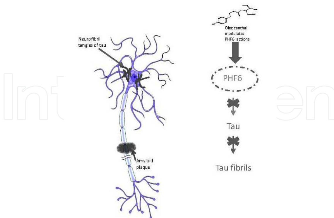
Fig. 4. Oleocanthal inhibits tau fibrilisation by covalently modifying the PHF-6 peptide which is crucial for the formation of tau fibrils. The fibrilisation of tau leads to neurofibrillary tangles which are inherently associated with neurodegenerative diseases such as Alzheimer's disease.
