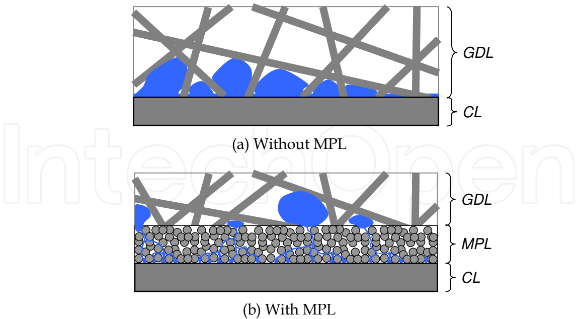
Fig. 13. Schematics of liquid water transport at the cathode CL | GDL interface without and with MPL
