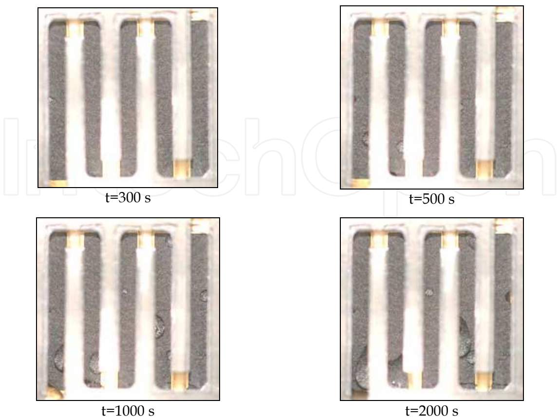
Fig. 6. Visualization images of liquid water behavior on the cathode GDL at 0.16 A/cm 2
