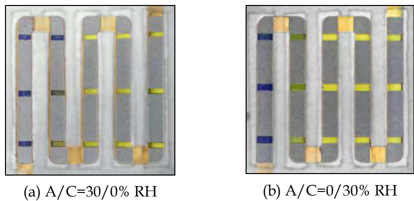
Fig. 20. Discoloration images of WSP in the anode channel for two different humidification conditions (Anode/Cathode(A/C)=30/0%, 0/30% RH) at high current density of 0.3 A/cm 2
