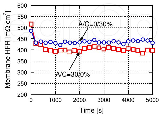
Fig. 21. Membrane HFRs for different humidification conditions (A/C=30/0%, 0/30% RH) at high current density of 0.3 A/cm 2
