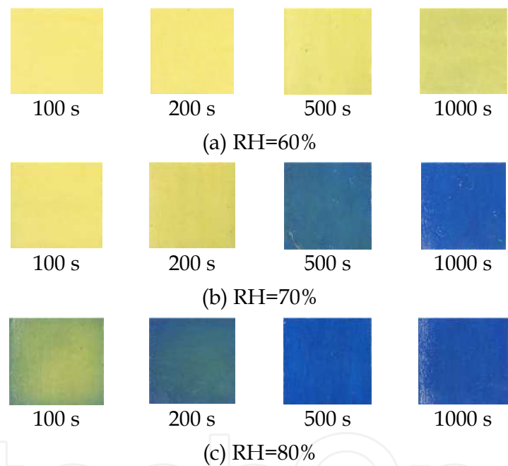
Fig. 15. Discoloration images of WSP when exposed to high humidity environments at 70°C
