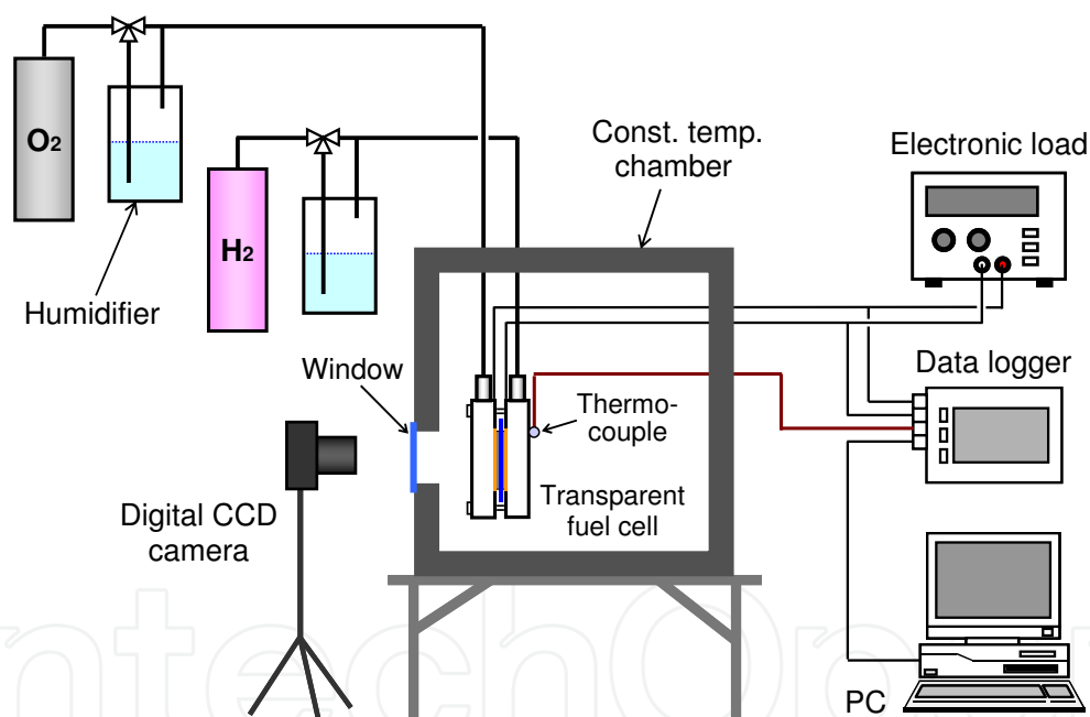
Fig. 2. Experimental setup used for PEFC operation test
