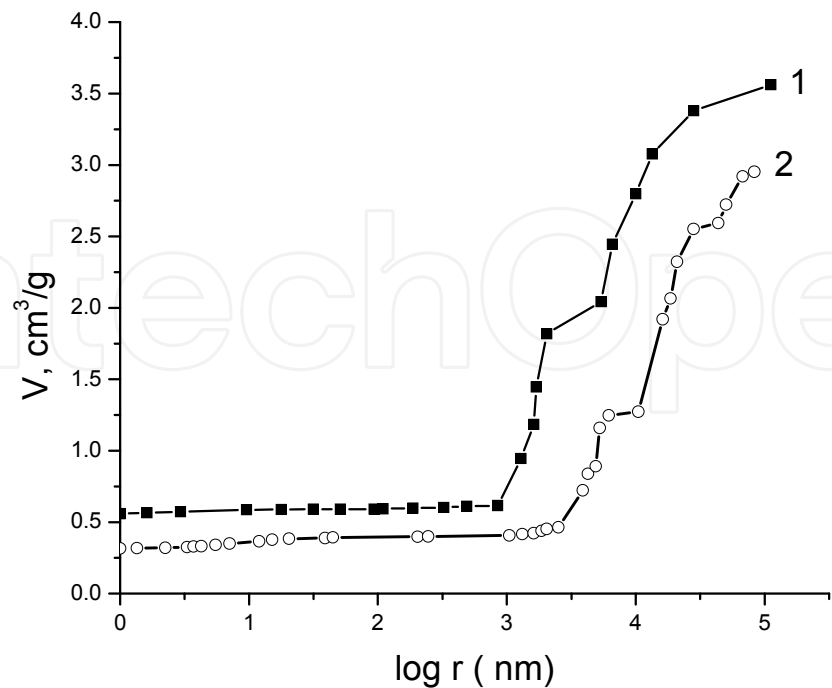
Fig. 4. Integral pore radius distribution curves measured in octane (1) and water (2) for a CH900-20 AC cloth.
