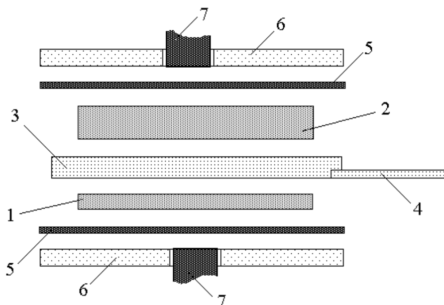
Fig. 3. Electrochemical group of the Teflon cell.
