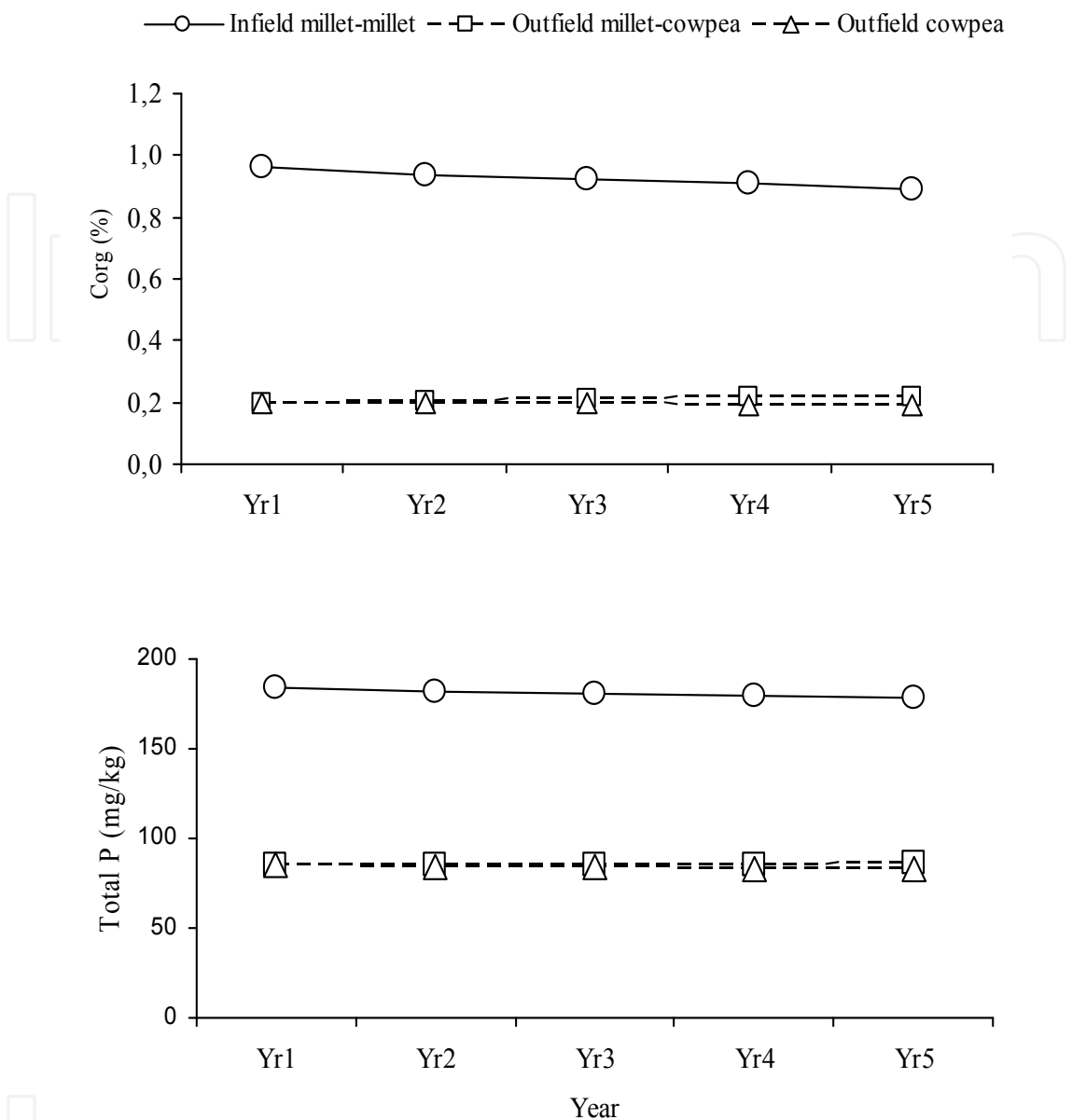
Fig. 2. Simulated evolution of soil organic matter and total P under different crop sequences on infields and outfields using the QUEFTS model (Janssen et al. 1990) (quantitative evaluation of the fertility of tropical soils). Solid lines refer to infields; dotted line to outfields, Soum province, Burkina Faso, 2004
