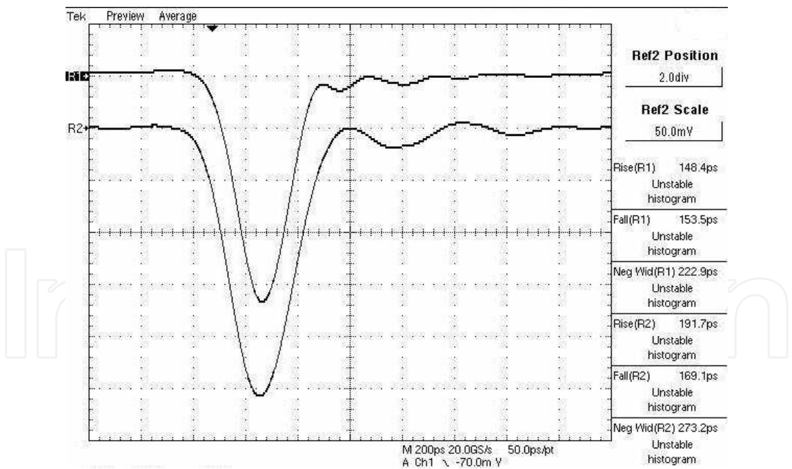
Fig. 16. Waveform of pulse response.
