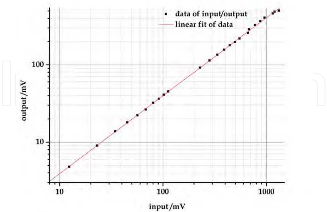
Fig. 17. Data and linear fitting curve of response.
