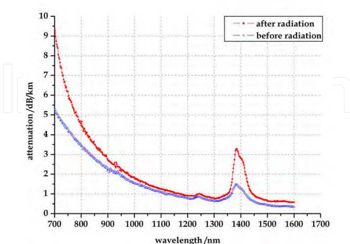
Fig. 21. Optical spectrum loss curve comparison before and after radiation exposure.
