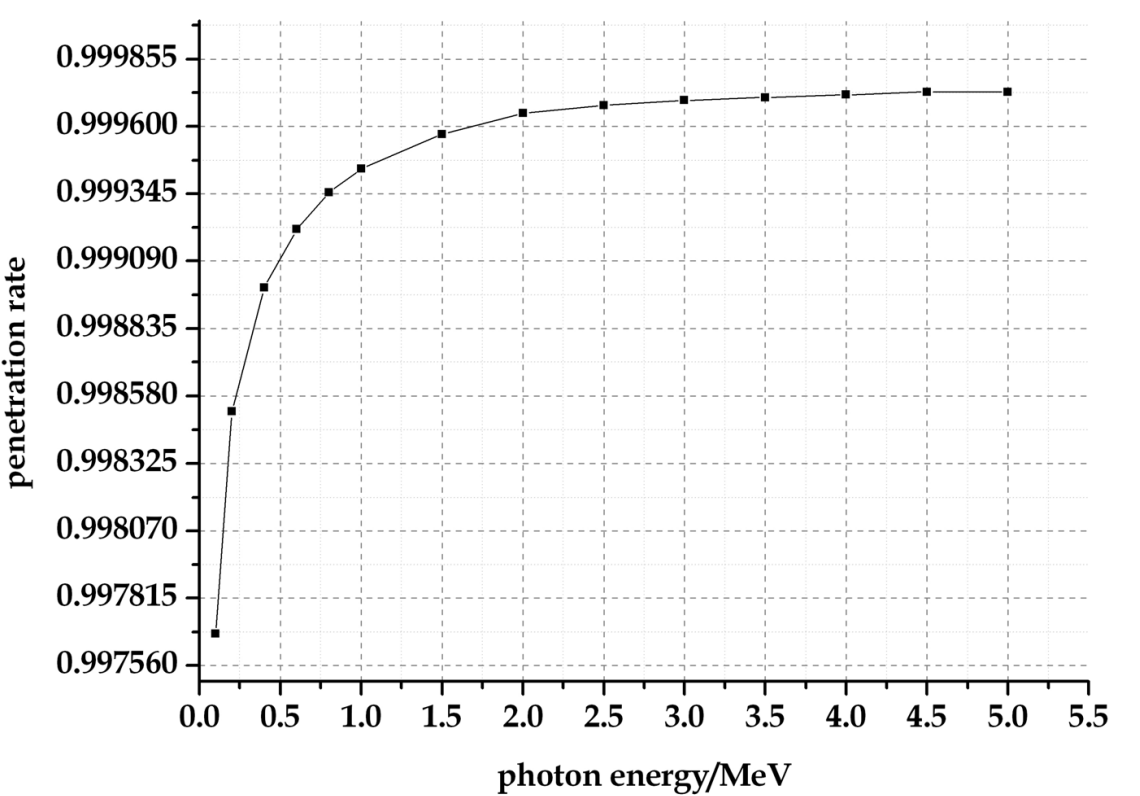
Fig. 2. Graph of penetration rate of γ-ray into optical fibers as a function of photo energy.
