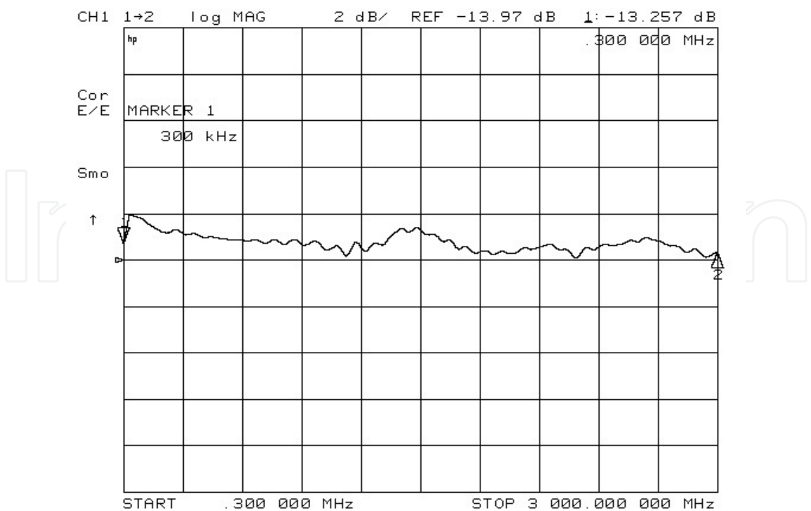
Fig. 15. Curve of amplitude-frequency characteristics.
